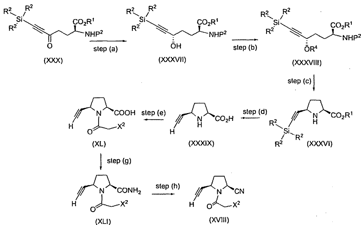
Scheme 7
