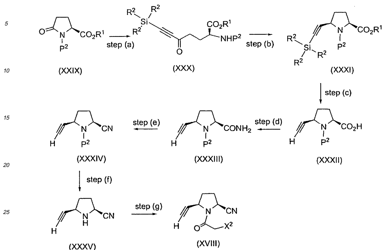
Scheme 6
