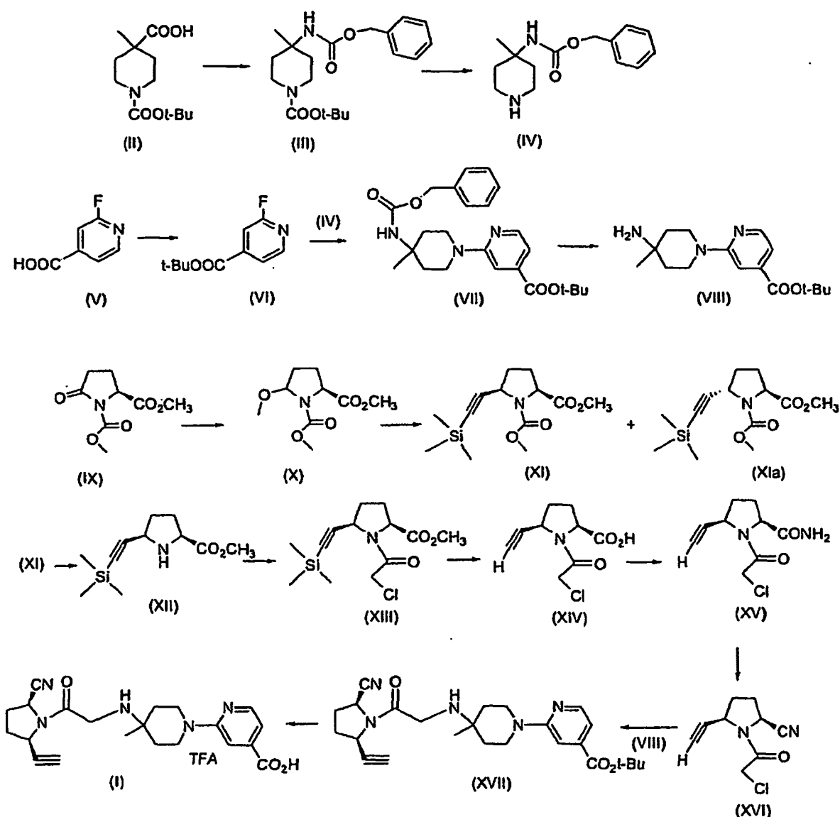
Scheme 1
