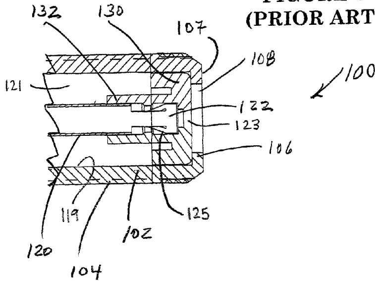
FIGURE 2 (PRIOR ART)
