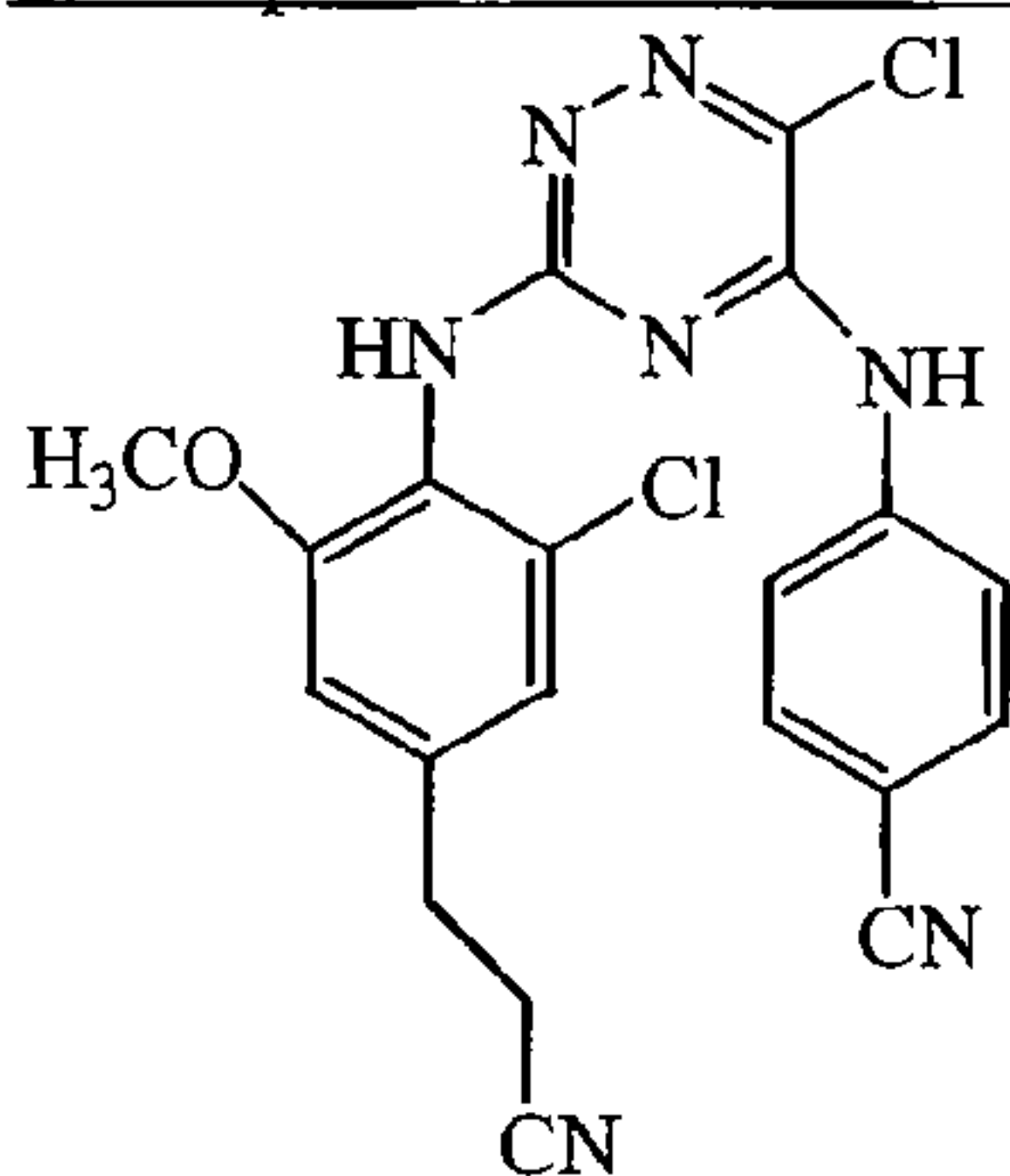
Intermediate 57
