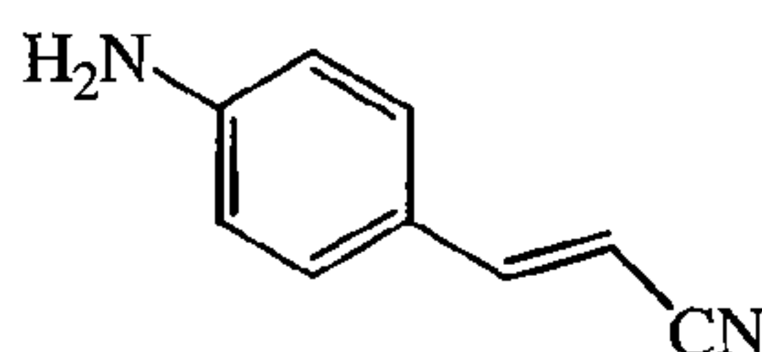
Intermediate 7
