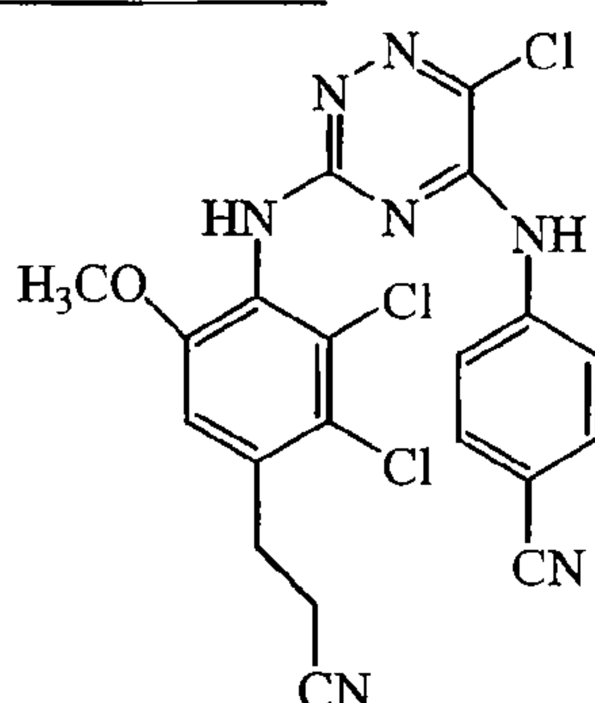
Intermediate 58
