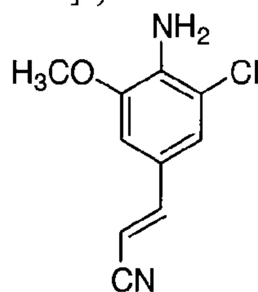
Intermediate 50
