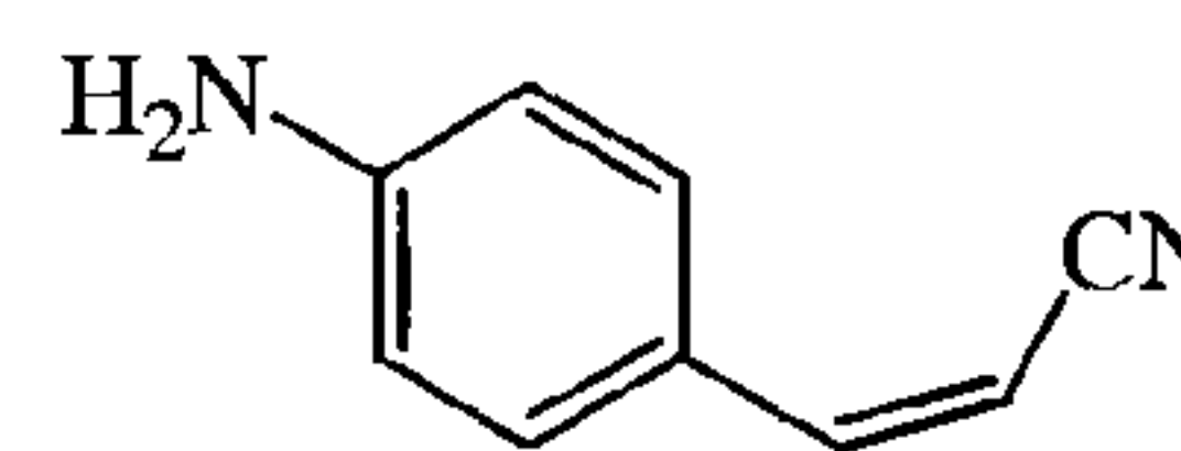
Intermediate 8
