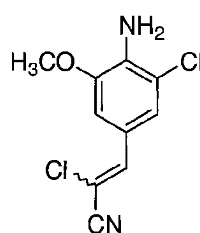
Intermediate 51
