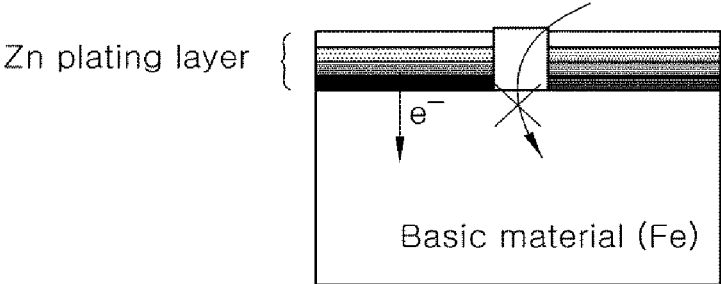
Protection mechanism of Zn Plating layer on Basic material (Fe)
