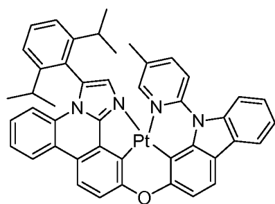
comparative compound 4
