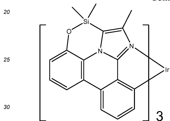
Compound 65
