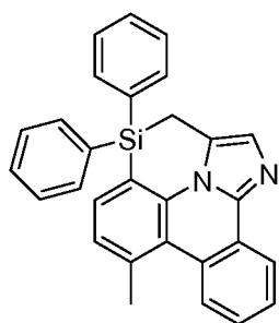
Compound (1-127)
