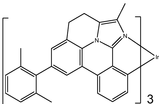
Compound 97
