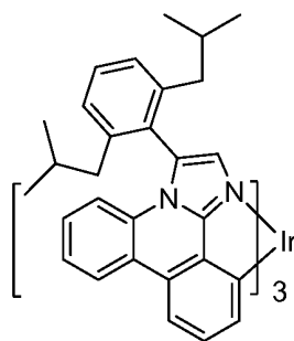
comparative compound 2
