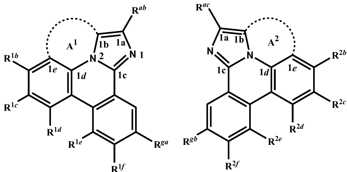
Formula (2a)
