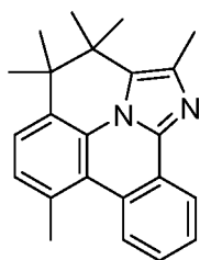
Compound (1-148)
