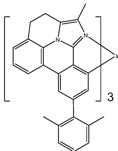
Compound 76
