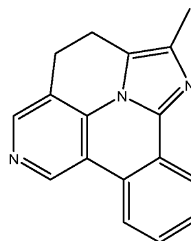
Compound (1-65)
