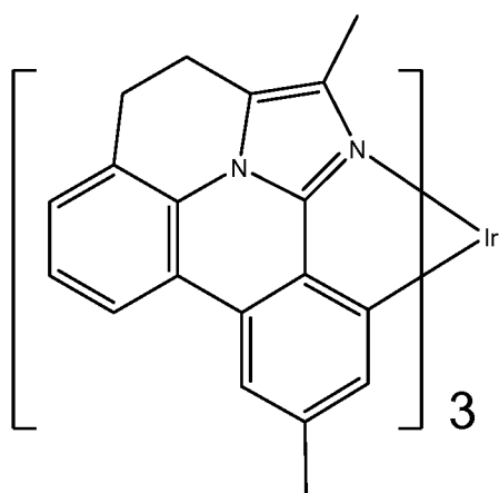
Compound 91
