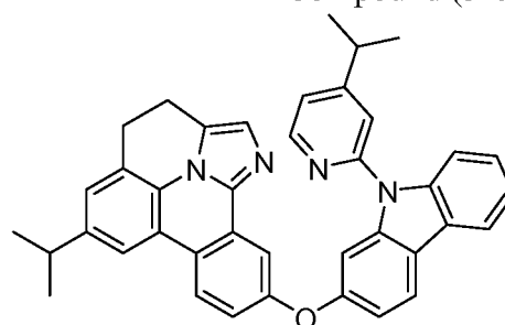
Compound (3-6)
