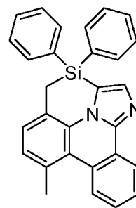
Compound (1-128)
