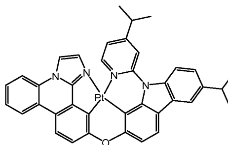
comparative compound 8
