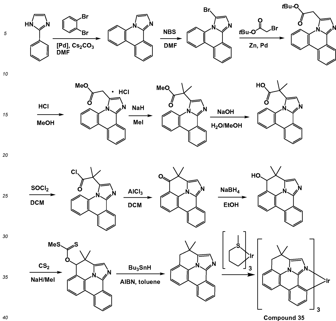
Scheme 5
