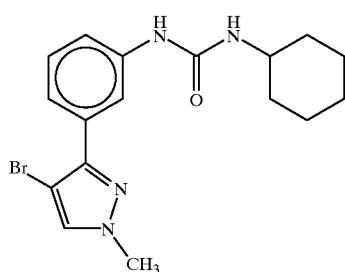
N-[3-(4-bromo-1-methylpyrazol-3-yl)phenyl] [cyclohexylamino]caboamide
