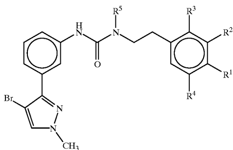
N-[3-(4-bromo-1-methylpyrazol-3-yl)phenyl] [(2-(4-methoxyphenyl)ethyl]amino]carboxamide
