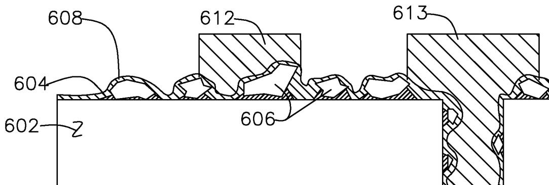
Figure 6F After Mask Strip
