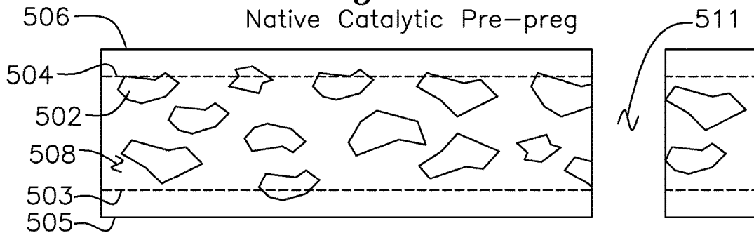
Figure 5B After etch & via drill
