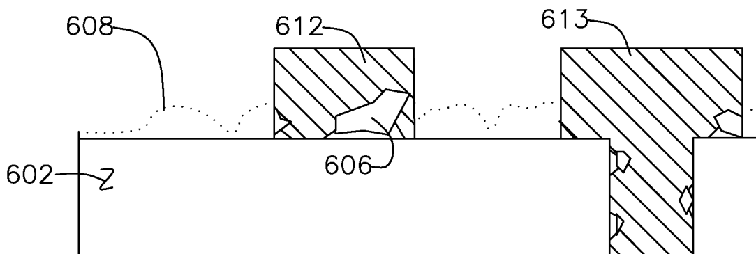
Figure 6G After quick Etch
