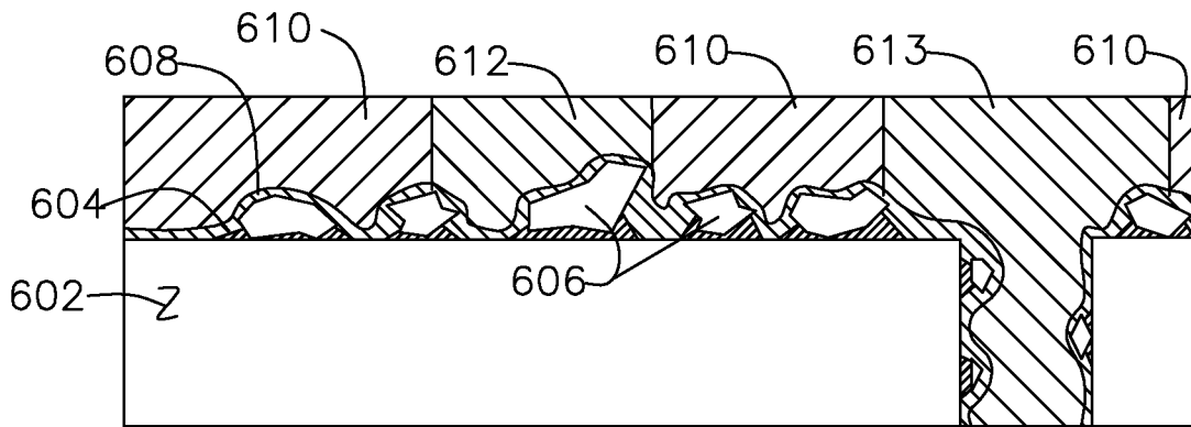
Figure 6F After Mask Strip
