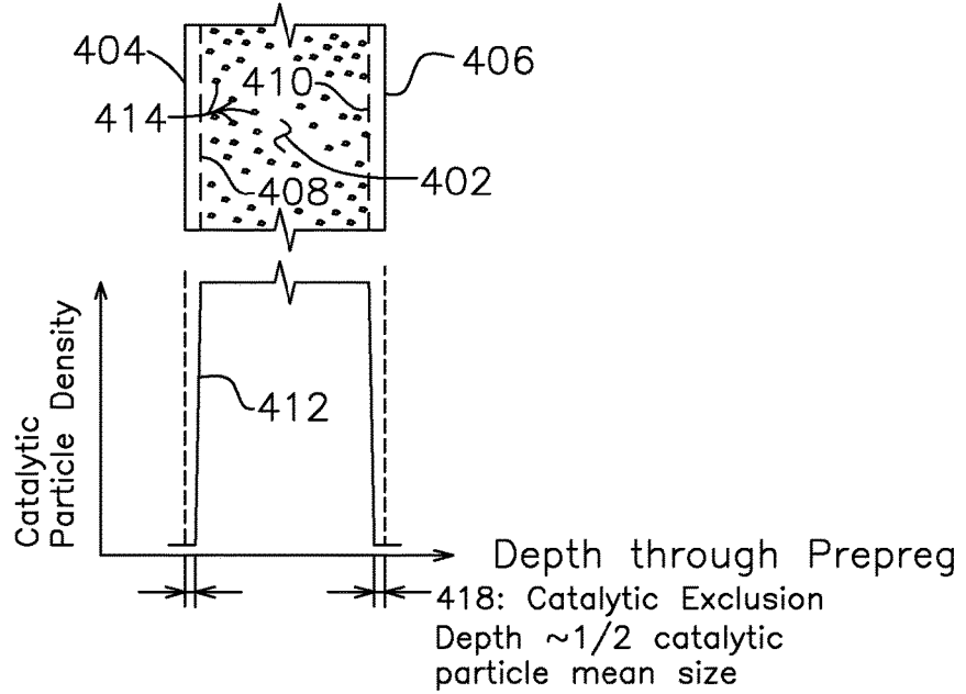
Figure 4 Catalytic Particle Distribution through Prepreg
