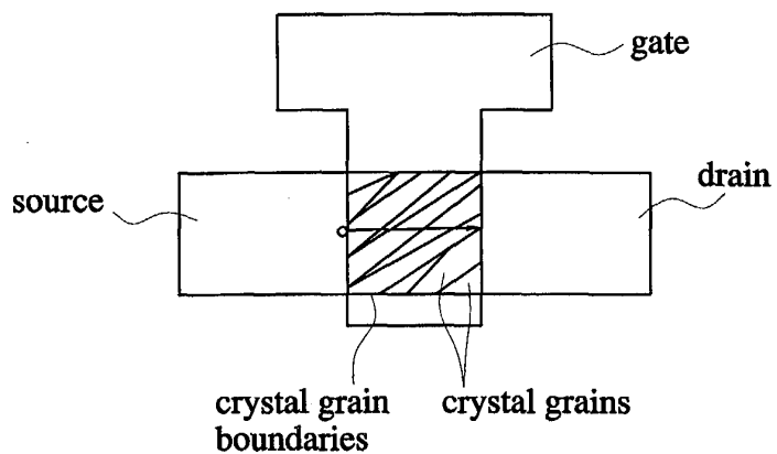
FIG. 3C (PRIOR ART)
