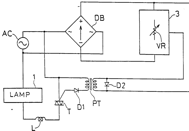
FIG. 6 (prior art)
