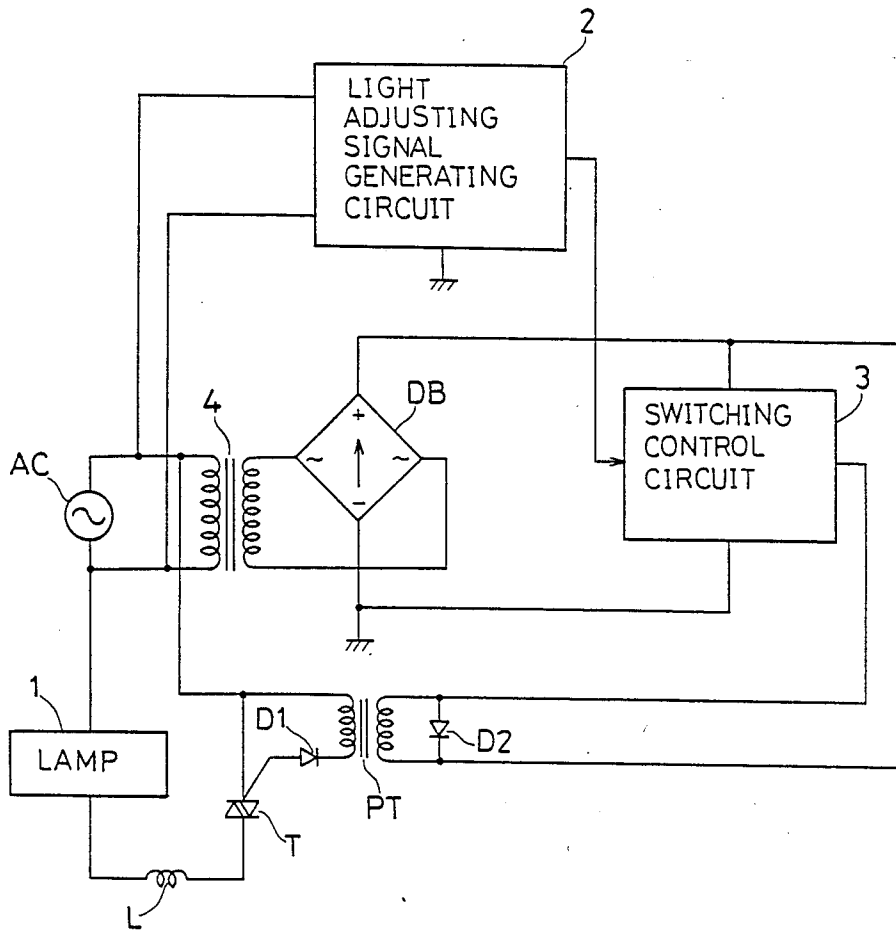
FIG. 7 (prior art)
