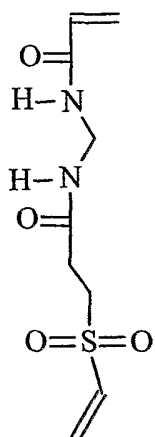
Monomer 2
