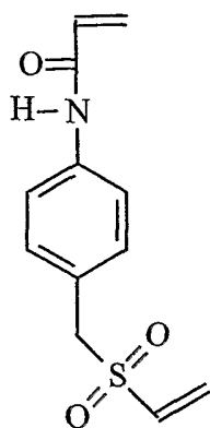
Monomer 1
