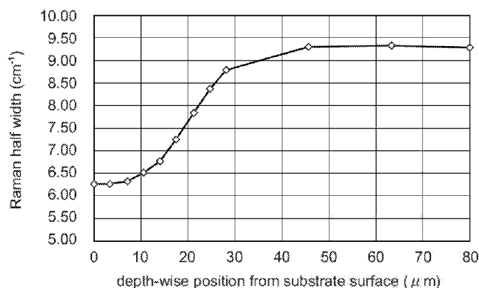
Raman profile
