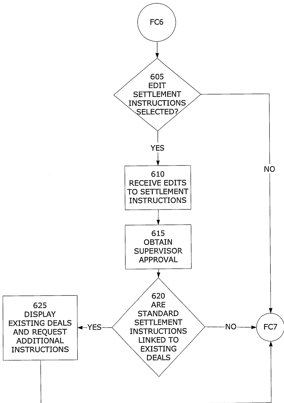
FIG. 6: SSI EDITING
