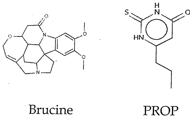
Figure 1 Structures of Brucine and PROP
