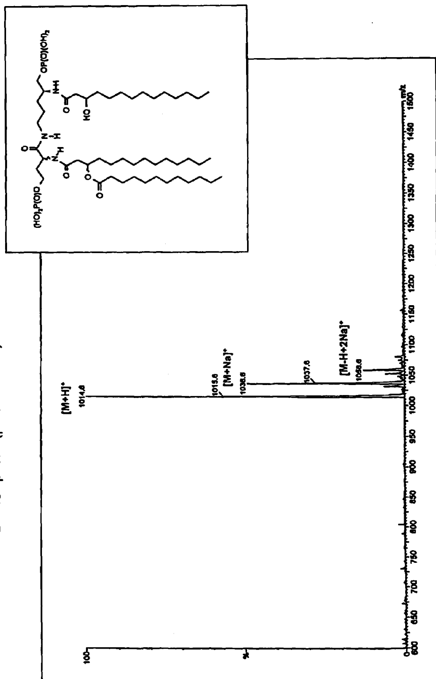
SPECTRUM 1 Diphosphorylated compound ES-MS spectra (positive mode) FIGURE 39
