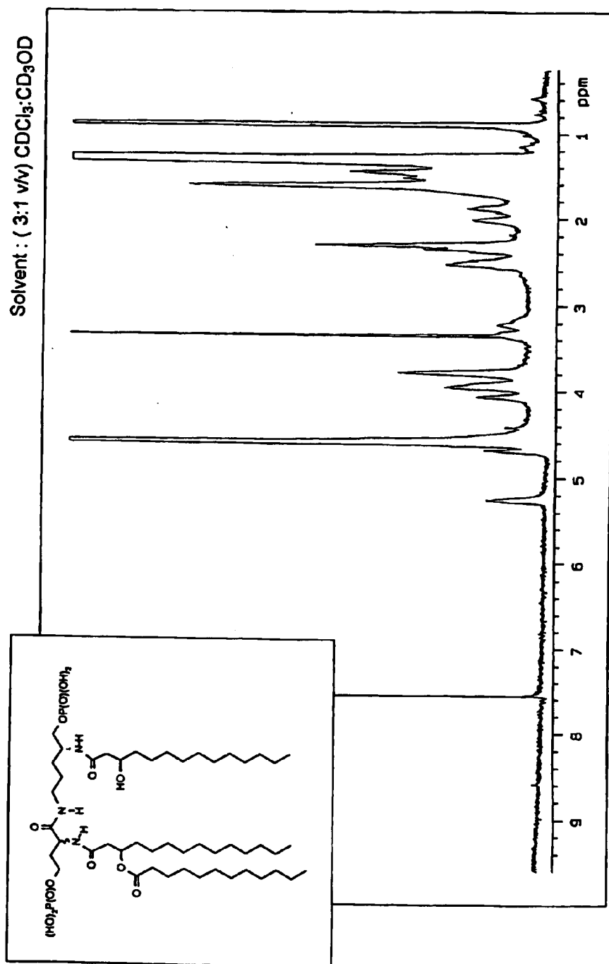
SPECTRUM 5 monophosphorylated compound 1 H-NMR Spectrum
