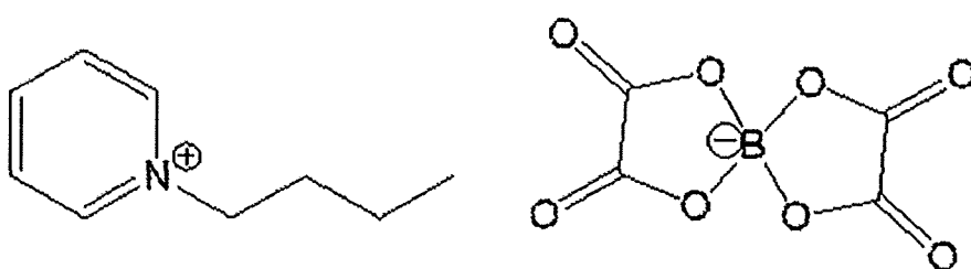
[Chem. 86]
