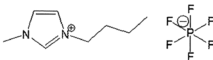
[Chem. 84]
