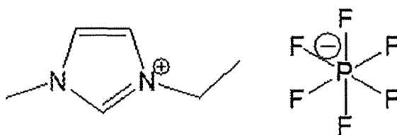
[Chem. 83]
