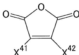
[Chem. 56]
