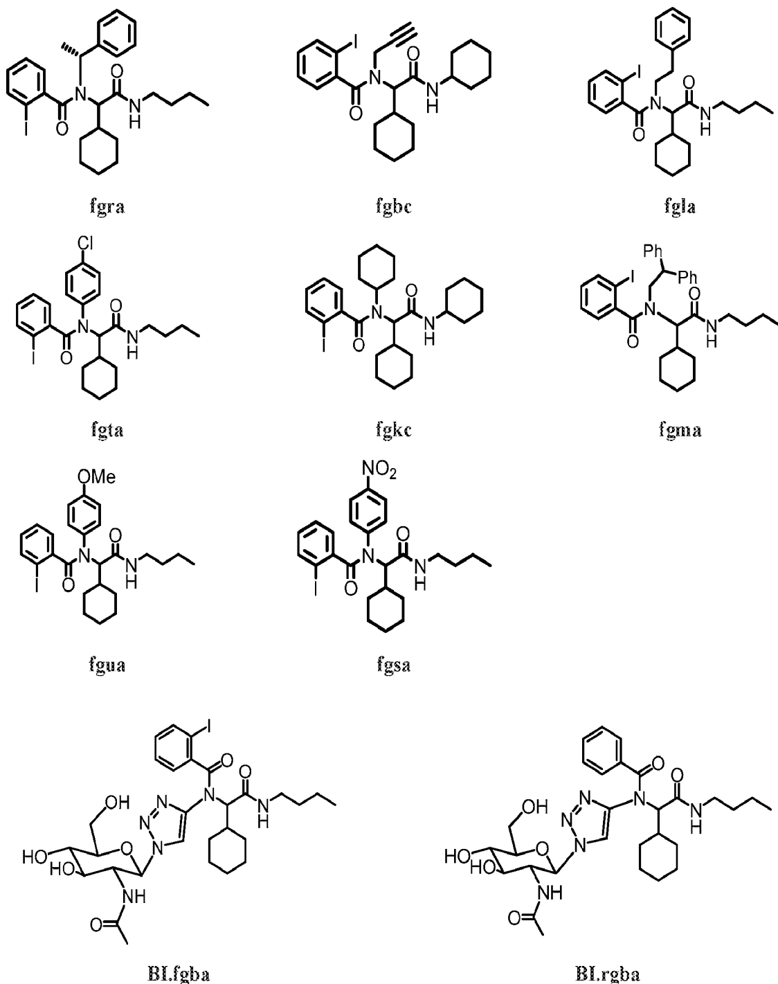
Scheme 14. GNT and Ugi-derived compounds used in resazurin microtiter assay.
