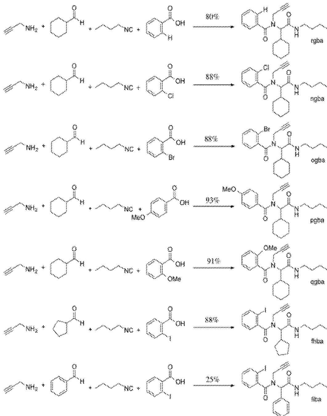
Scheme 4. Synthesis of Ugi compounds; varied substituents highlighted in red.
