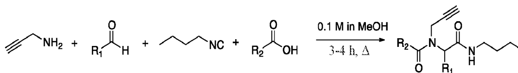
Scheme 2. General Ugi reaction using propargyl amine and n-butyl isocyanide.
