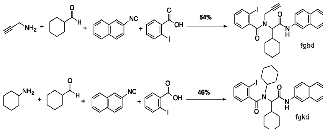
Scheme 12. Ugi reaction synthesis of fgbd and fgkd
