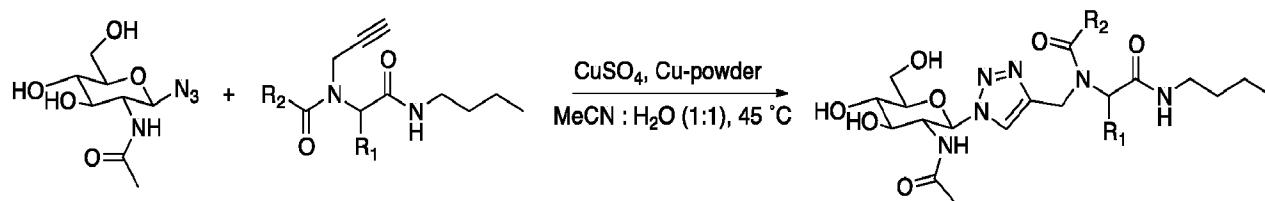
Scheme 7. General synthesis of GNT products.
