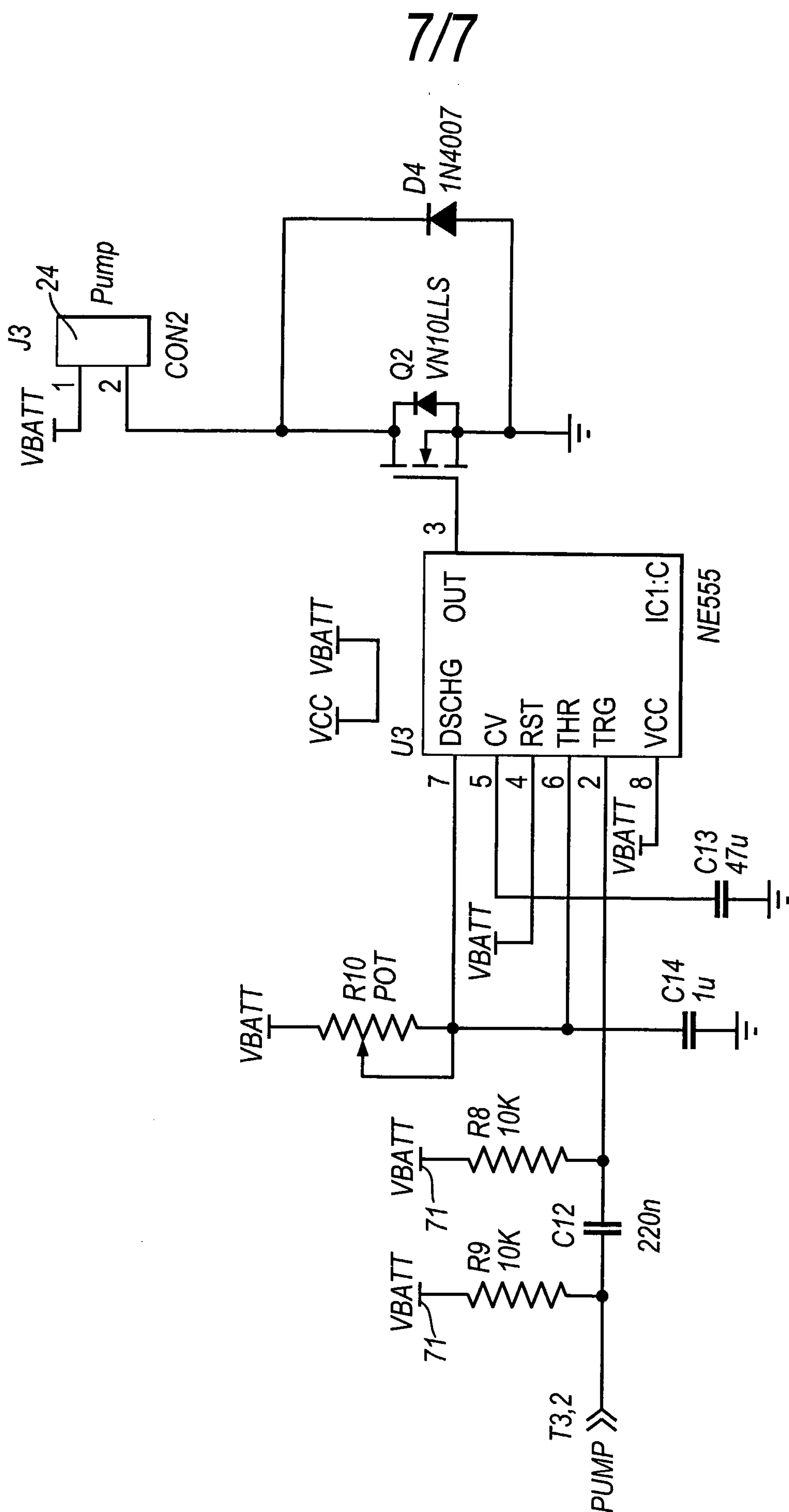
Fig. 9 Pulse Generator and Pump Drive
