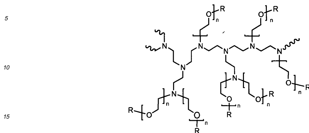
formula (I)
