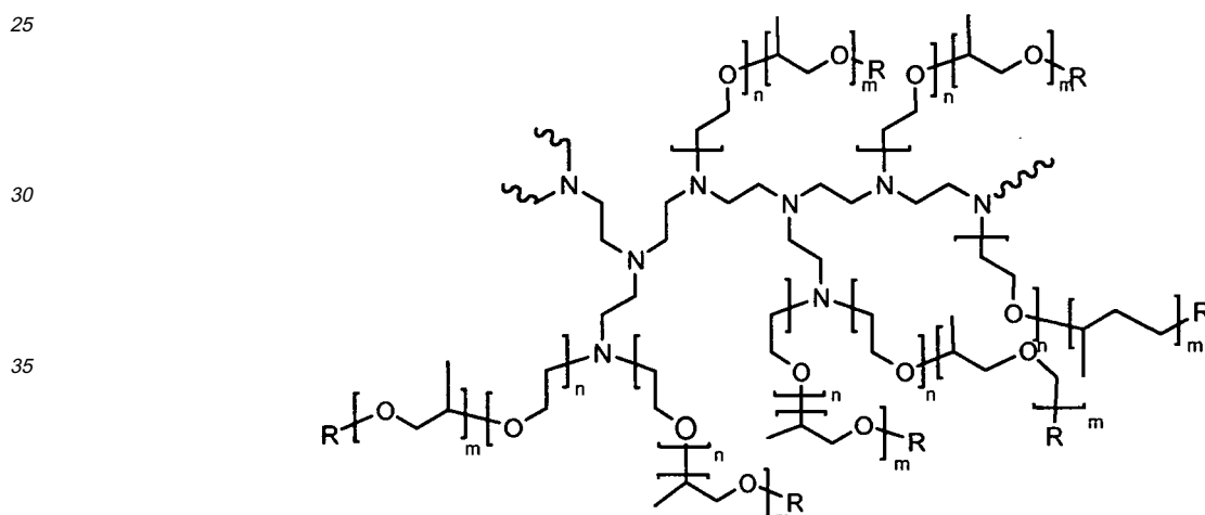
formula (II)
