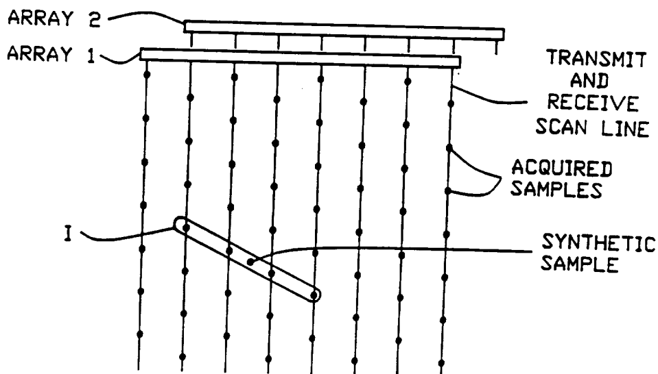
LINEAR SCAN FORMAT (HEXAGONAL COORDINATE SAMPLING)
