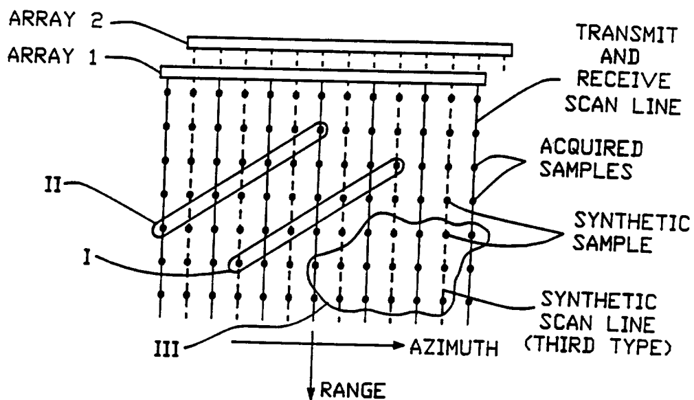
LINEAR SCAN FORMAT (CARTESIAN COORDINATE SAMPLING)
