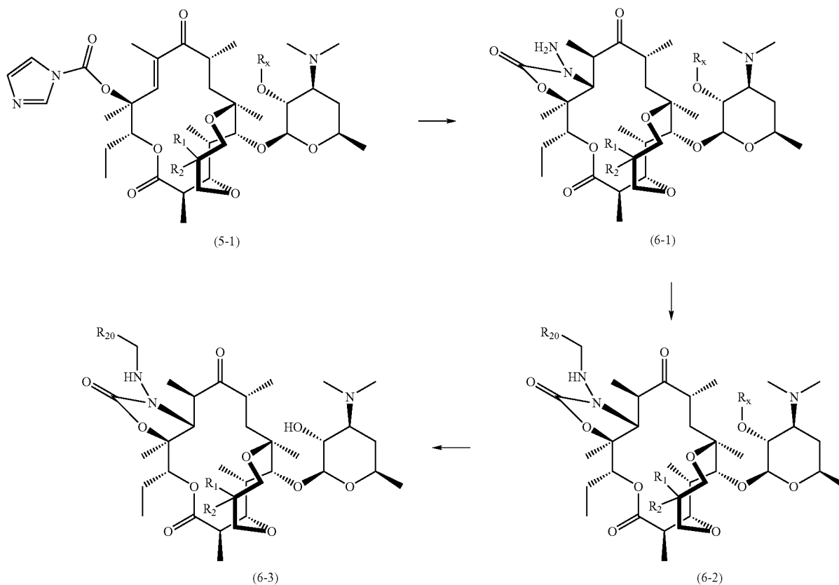
Scheme 6
