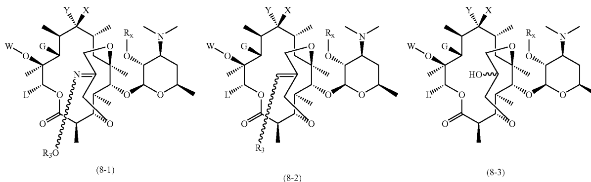
Scheme 8
