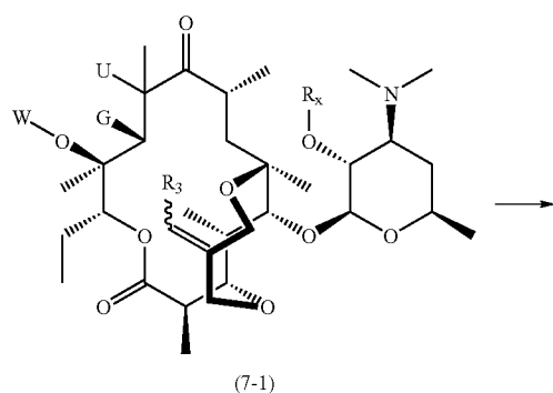
Scheme 7
