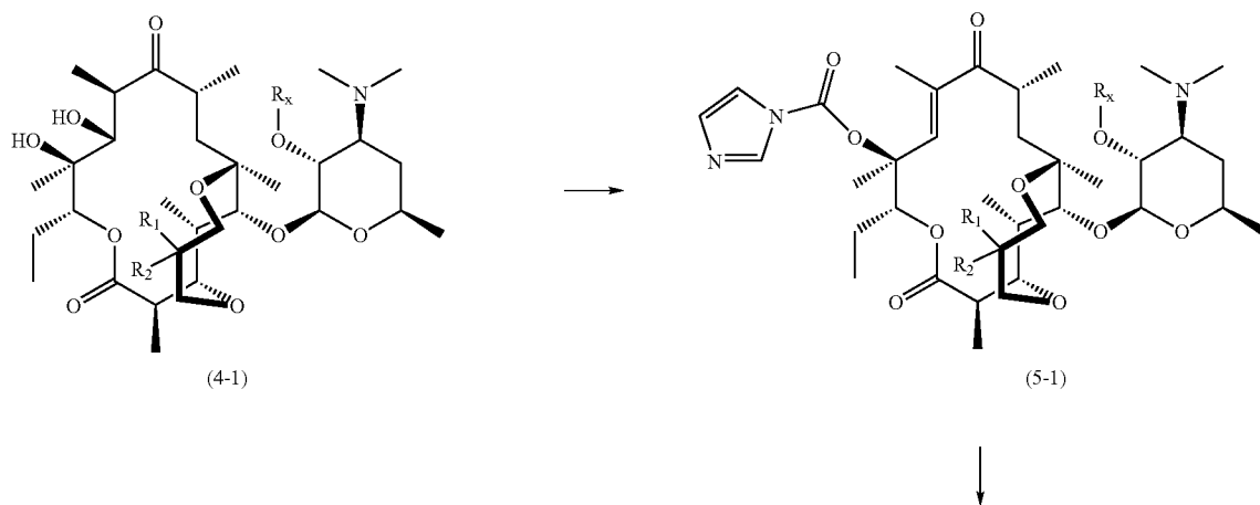
Scheme 5
