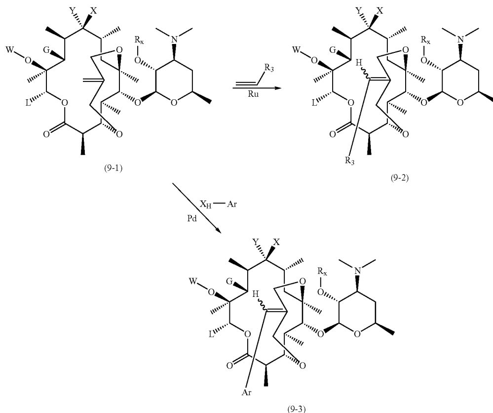
Scheme 9
