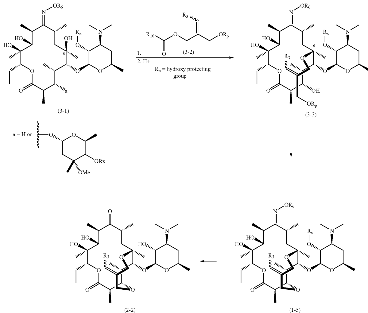
Scheme 3
