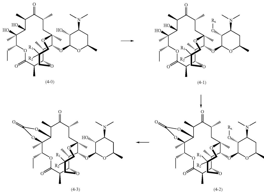
Scheme 4
