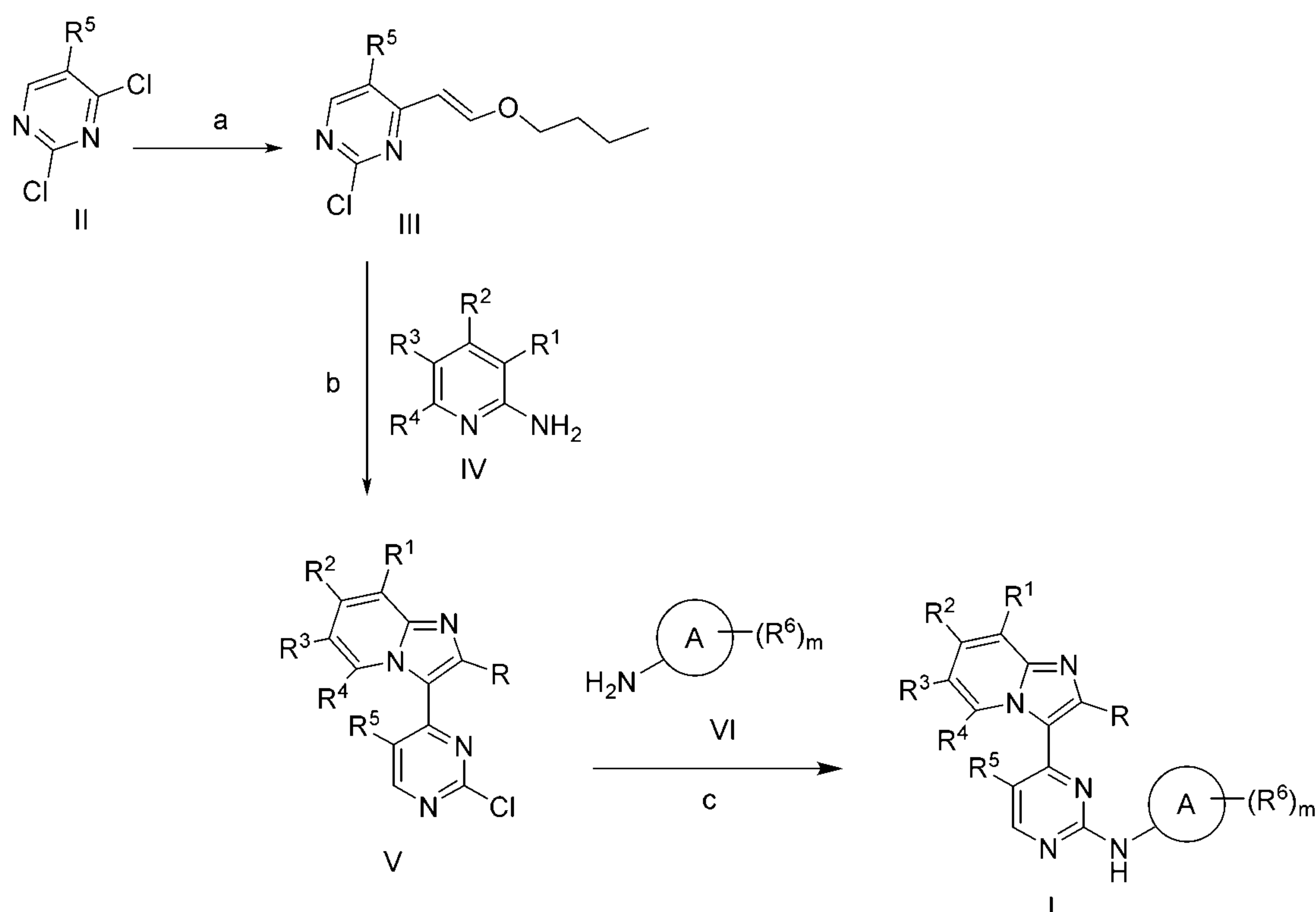
Scheme 1
