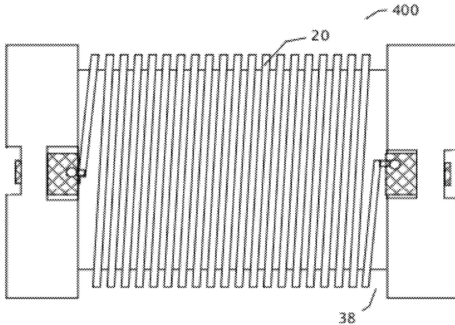
Figure 48. Top view.
