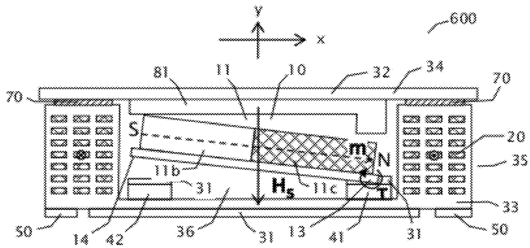
Figure 6. Front view.
