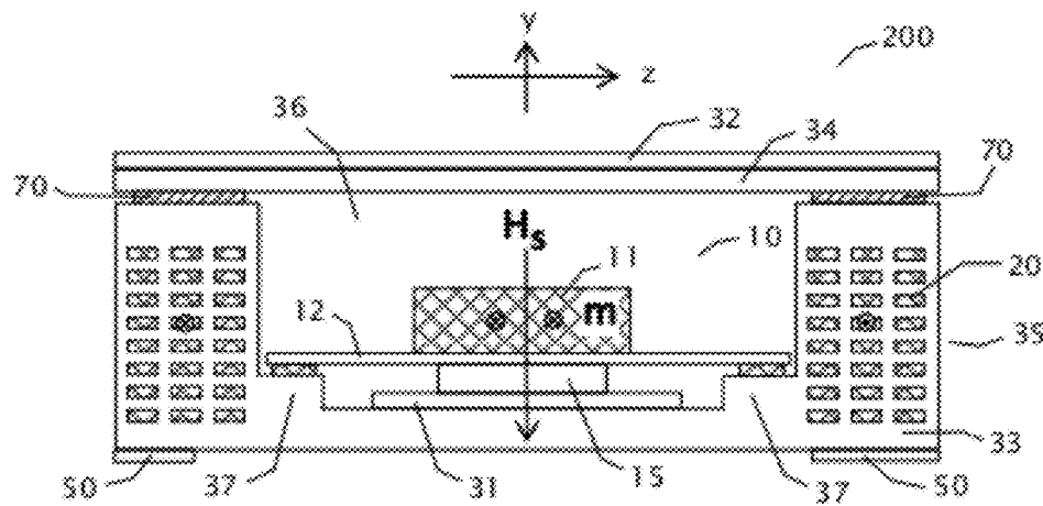
Figure 28. Side view.
