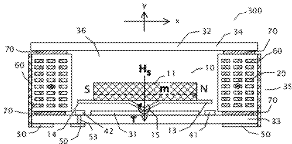
Figure 3. Front view.
