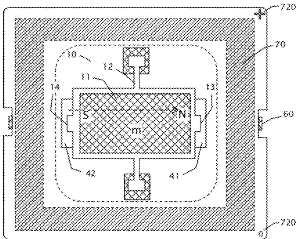
Figure 18. Top view.
