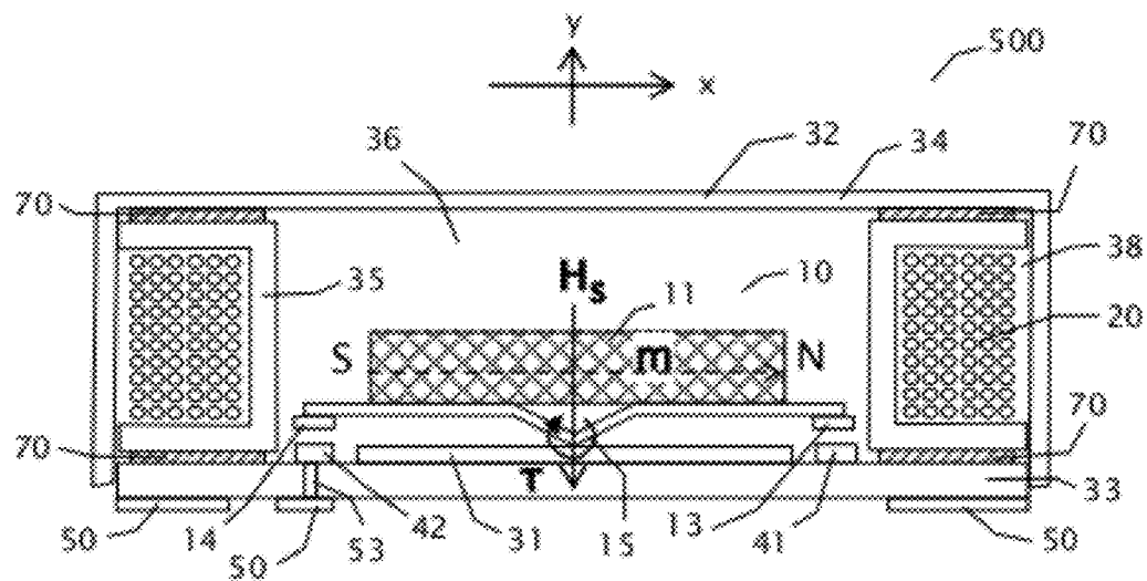
Figure 5. Front view.
