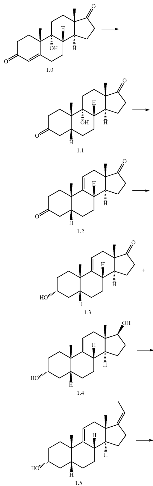
Scheme 1. Synthesis of Deoxycholic Acid (DCA)
