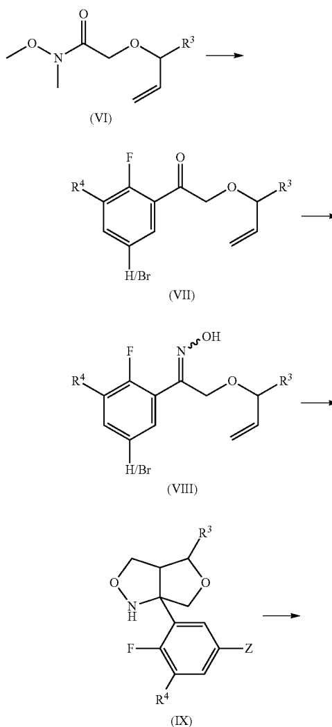
Reaction scheme 3
