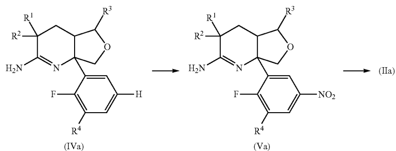
Reaction scheme 2
