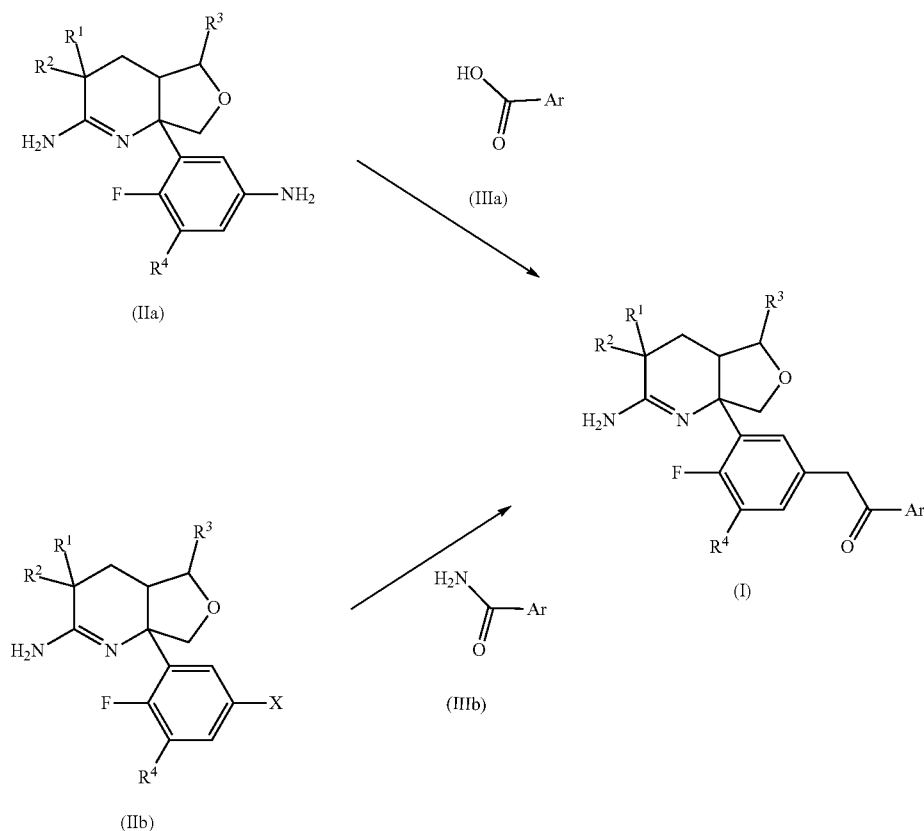
Reaction Scheme 1
