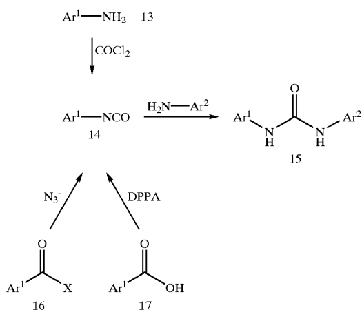
Scheme IV Selected Methods of Non-Symmetrical Urea Formation
