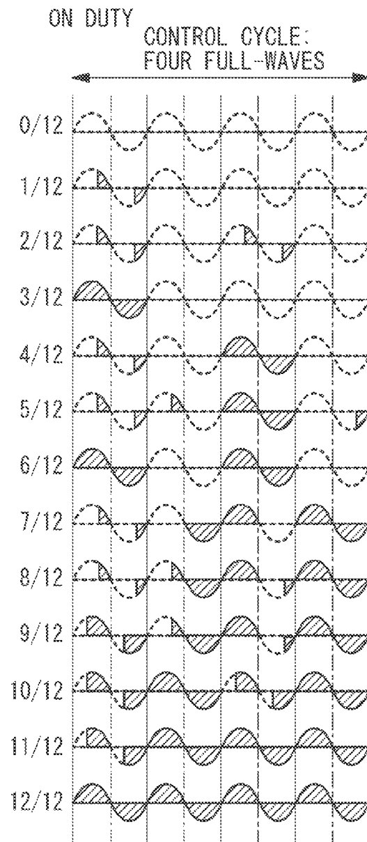
FIG. 1B <AT HIGH TEMPERATURE>
