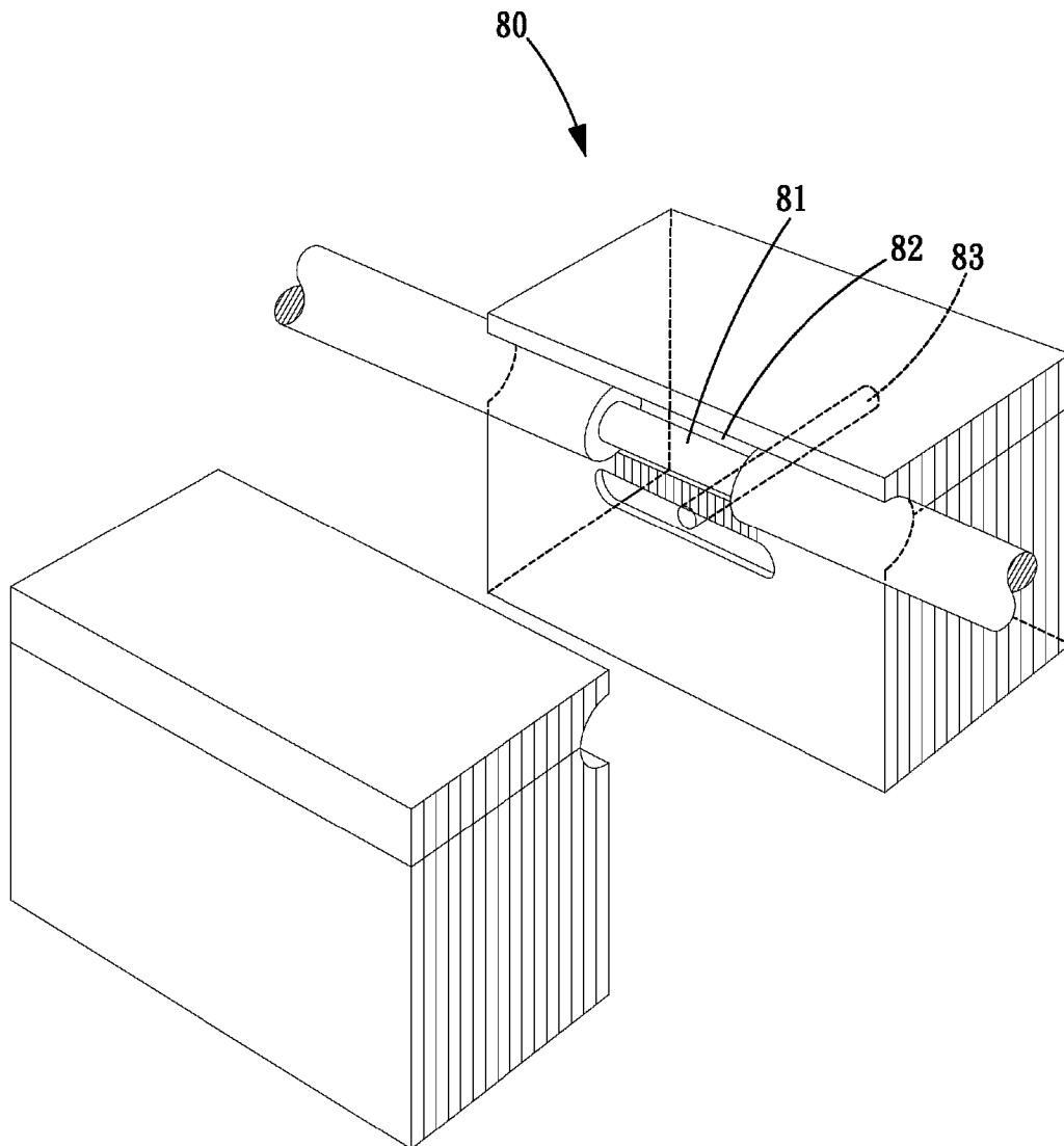
FIG. 5 PRIOR ART
