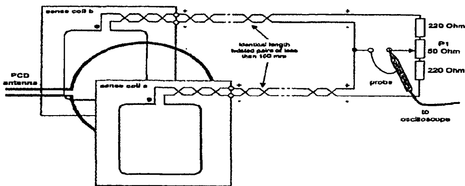
Test set-up (principle)
