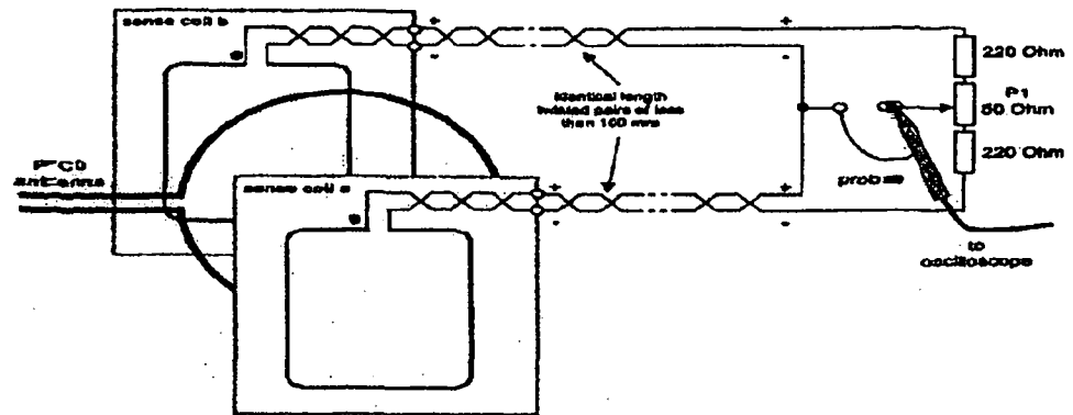
Figure 1 — Test set-up (principle)
