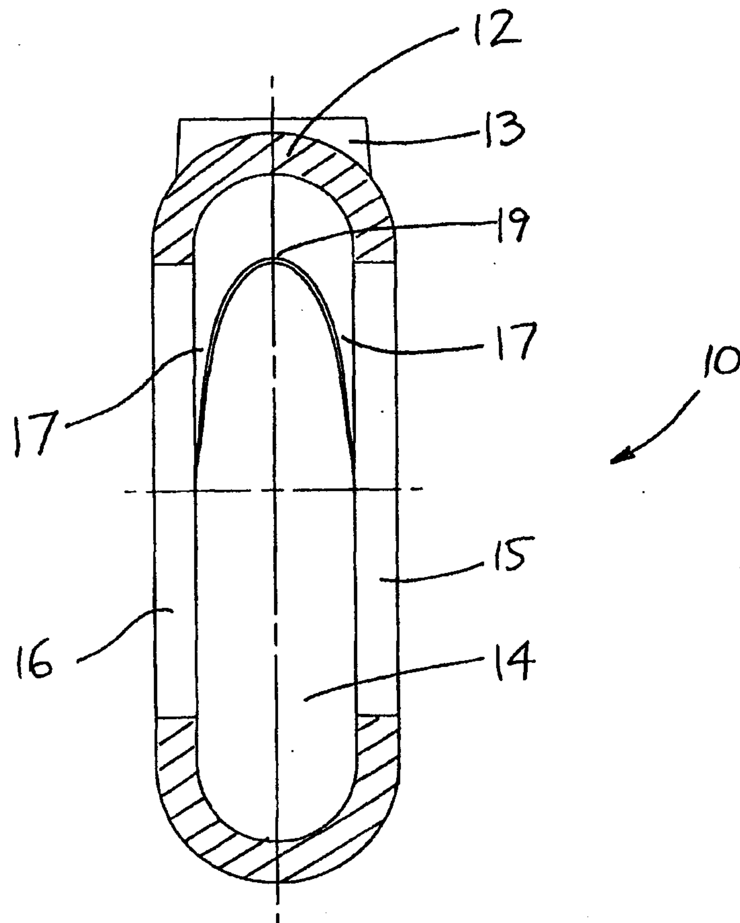
FIG. 4 (PRIOR ART)
