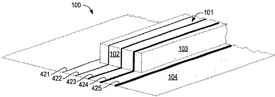
FIG. 6 PRIOR ART
