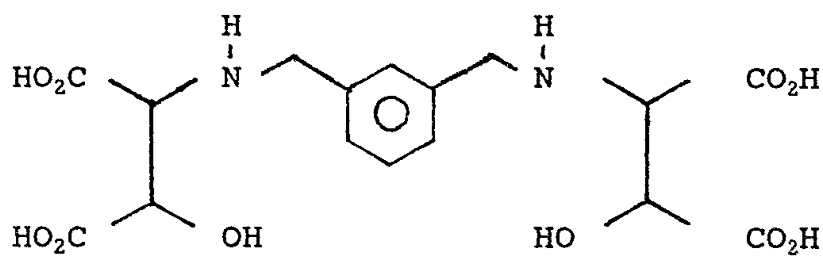
Compound 4
