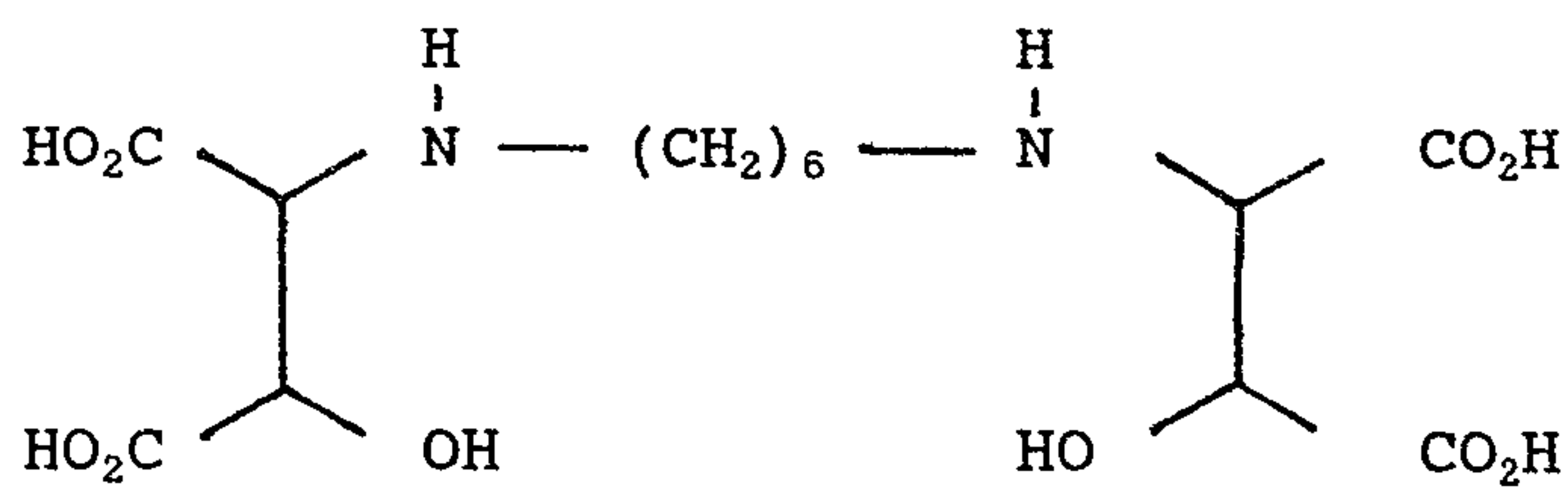
Compound 3
