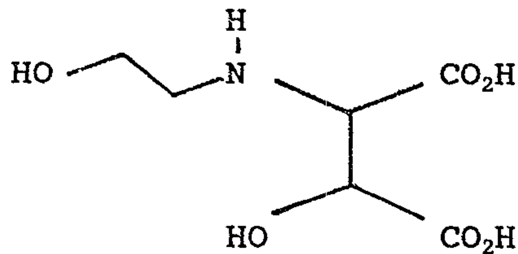
Compound 2
