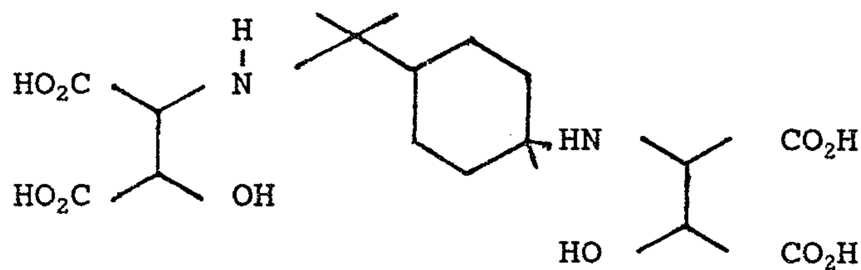
Compound 4
