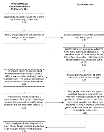
Example Implementation Using Product Widgets
