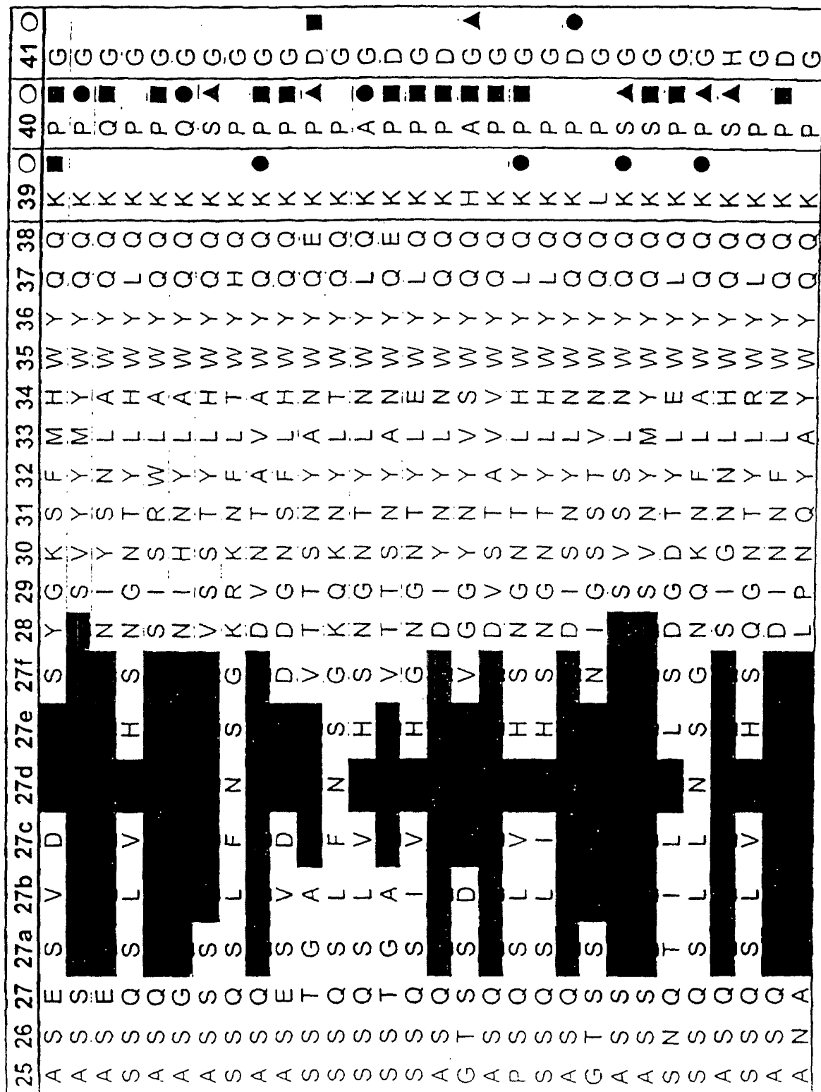
Figure 2a: Variable/constant domain interface residues for VL (cont.)
