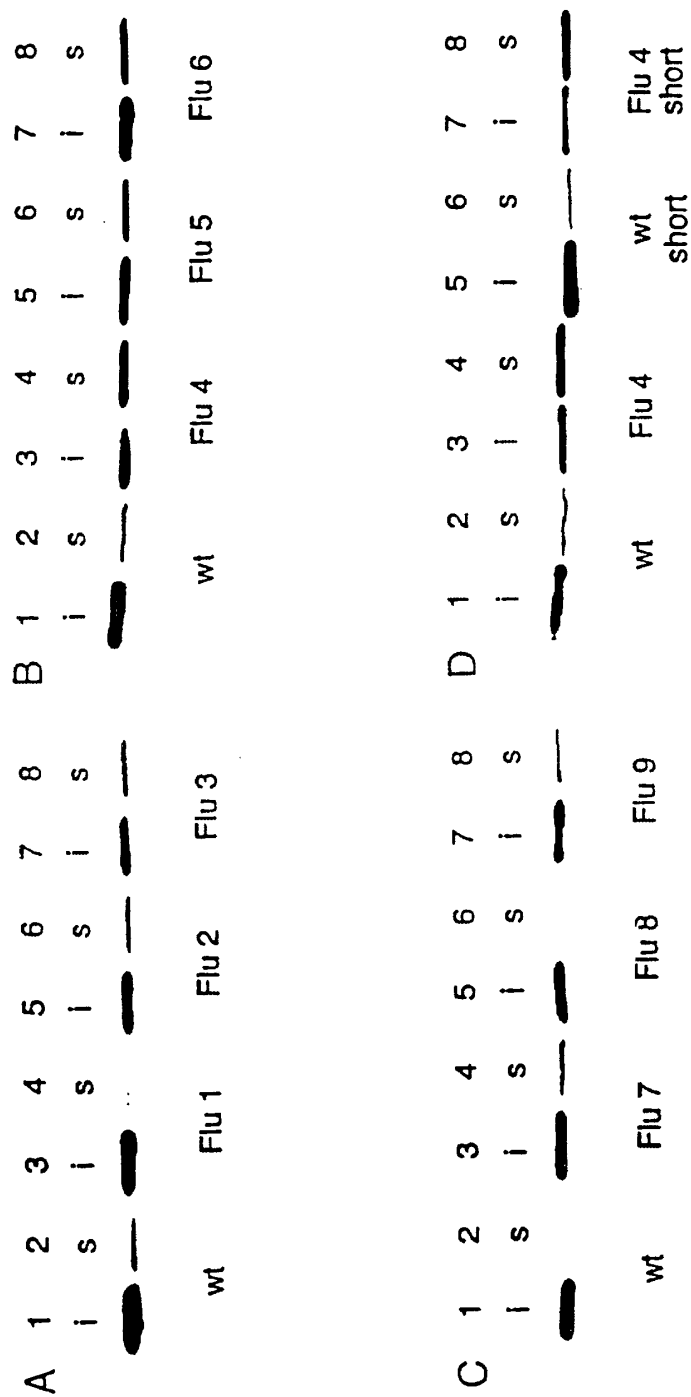
Figure 3: Western blots showing the insoluble (i) and soluble (s) fractions of cell extracts
