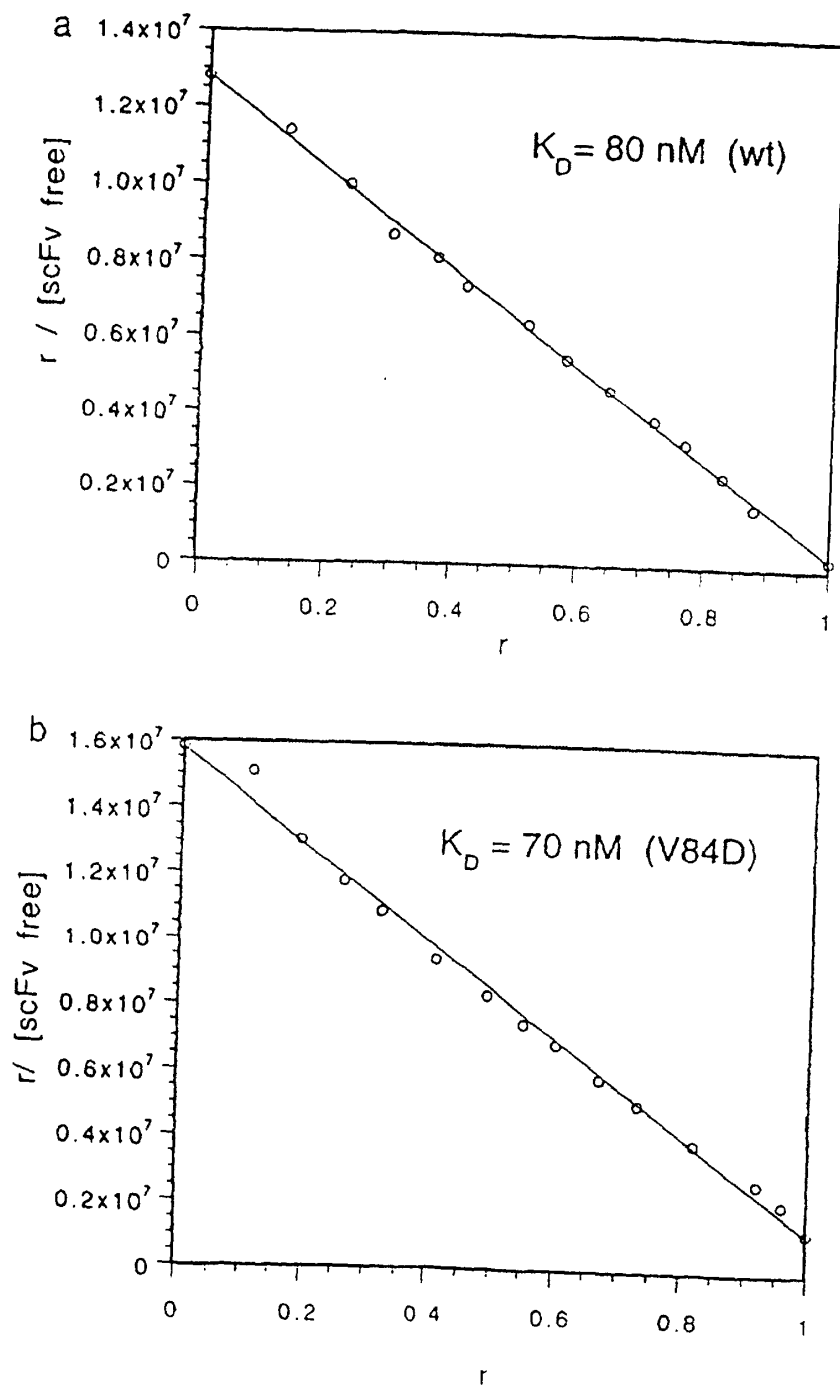
Figure 4: Scatchard plots of fluorescence titration of fluorescein with antibody: a) Titration of wt scFv; b) Titration of Flu4(V84D)
