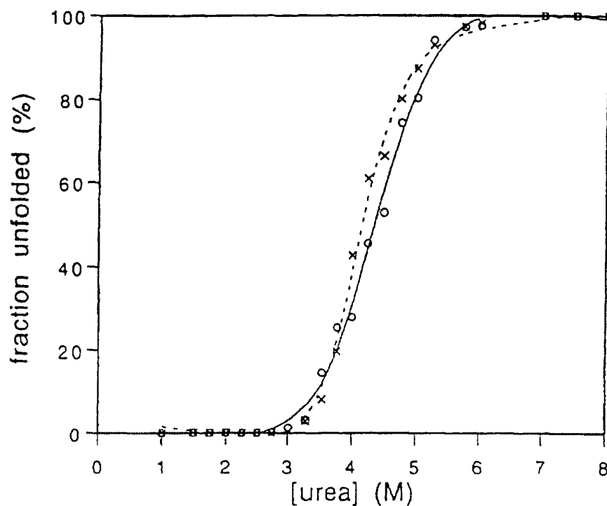
Figure 5: Overlay plot of urea denaturation. (x) wt scFv, (o) Flu4
