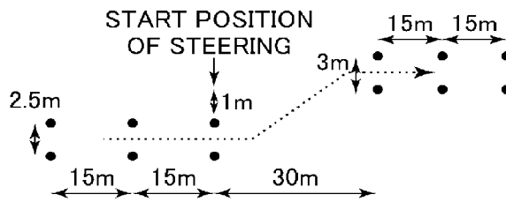
FIG.30B SINGLE LANE CHANGE
