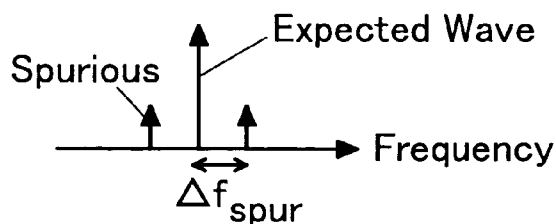
GSM Spurious
