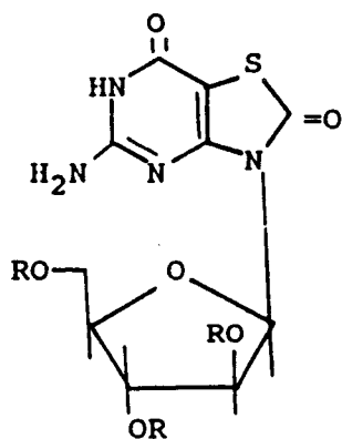
39 R = Benzyl 40 R = H
