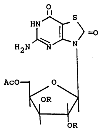
37 R = Acetyl 38 R = H
