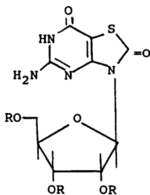
41 R = Acetyl
