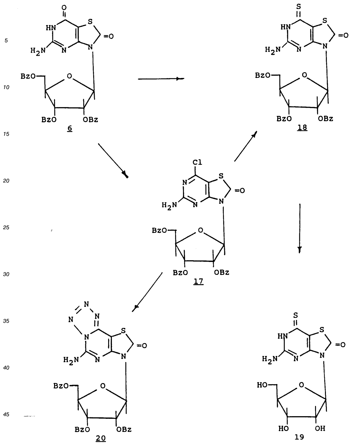
SCHEME III
