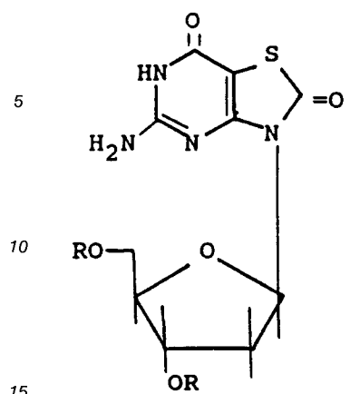
35 R = Toluoyl 36 R = H
