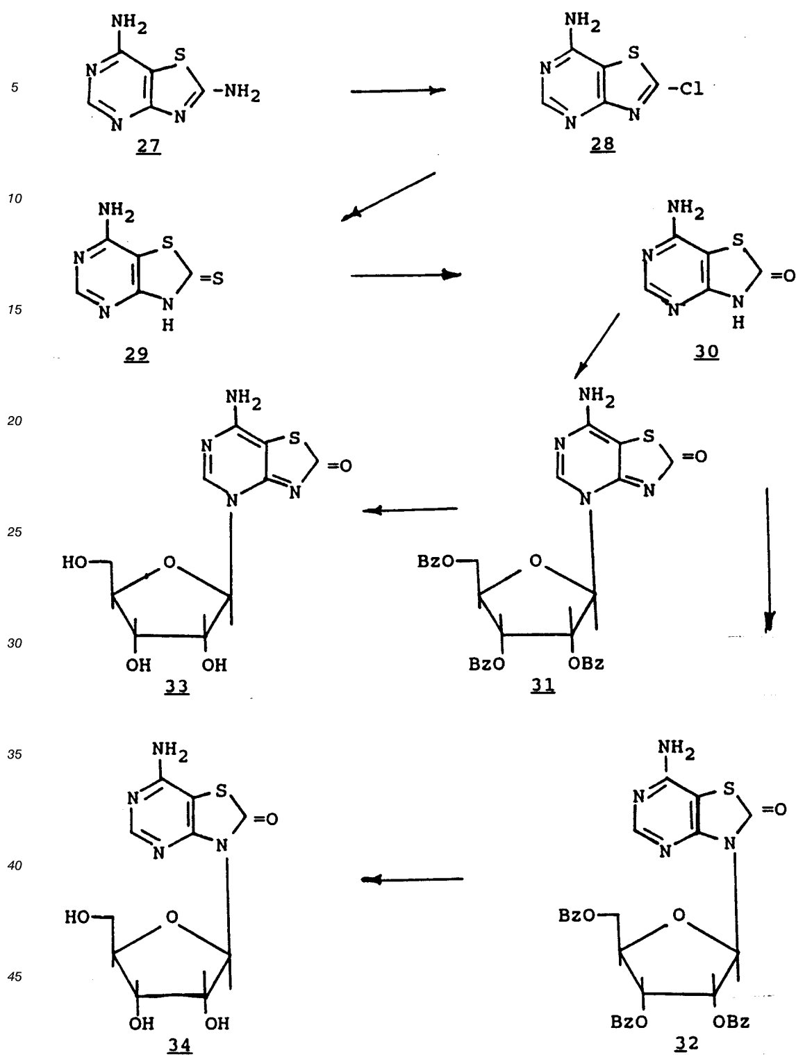
SCHEME V
