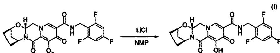
Compound G1-a
