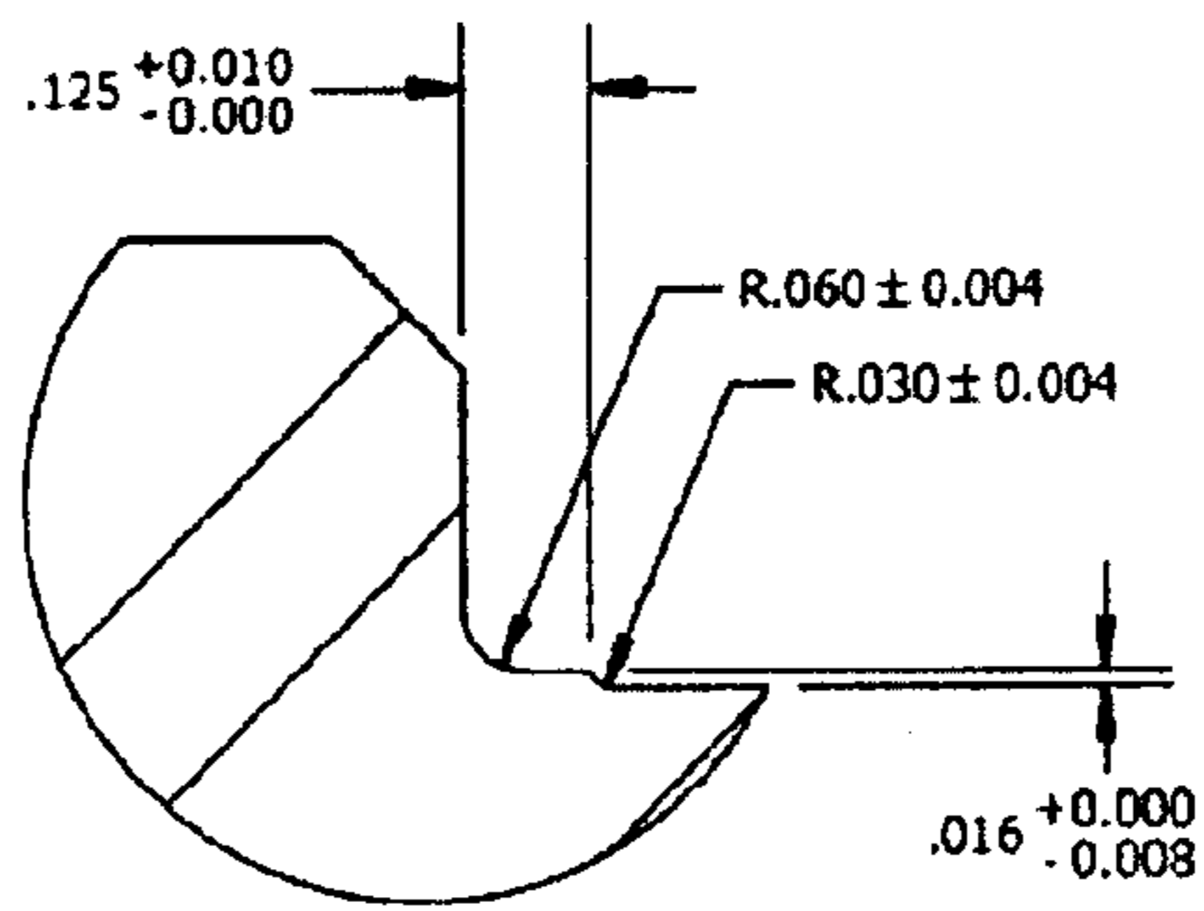
DETAIL B SCALE 2 : 1
