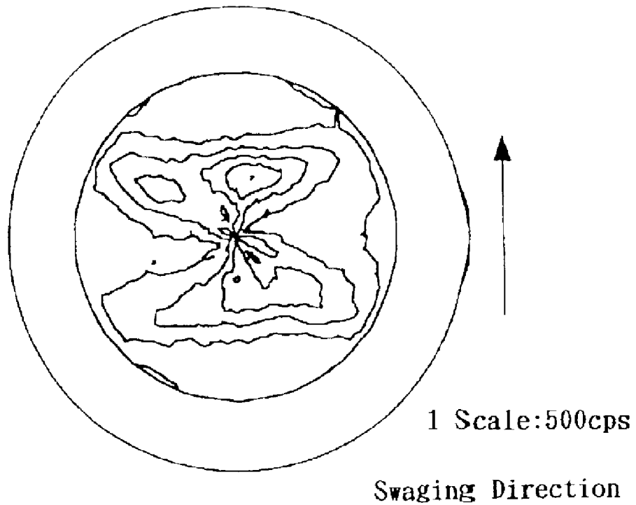
(110) Polar Figure Obtained in Comparative Sample
