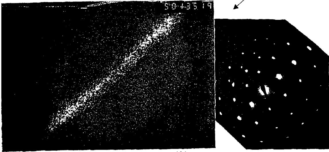
TEM Observation Result in Sample No. 1 Electron Diffraction Pattern and Dark Field Image Using 110 Diffraction Point Value read by goniometer was -16.3^\circ .
