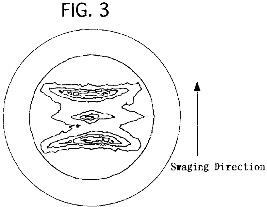
(110) Polar Figure Obtained in Sample No. 1
