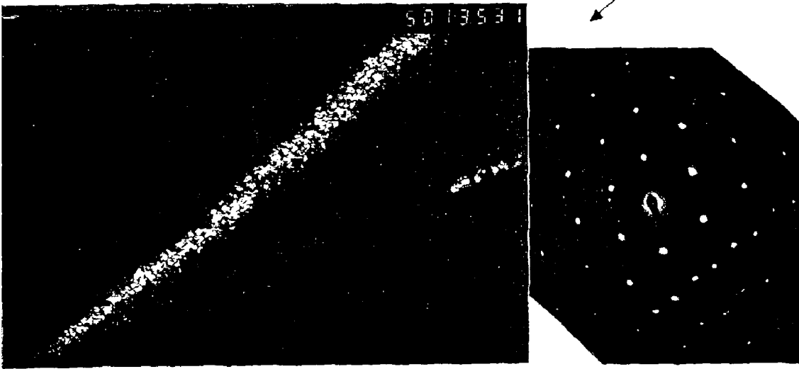
TEM Observation Result in Sample No. 1 Electron Diffraction Pattern and Dark Field Image Using 110 Diffraction Point Value read by goniometer was 6.1^\circ .
