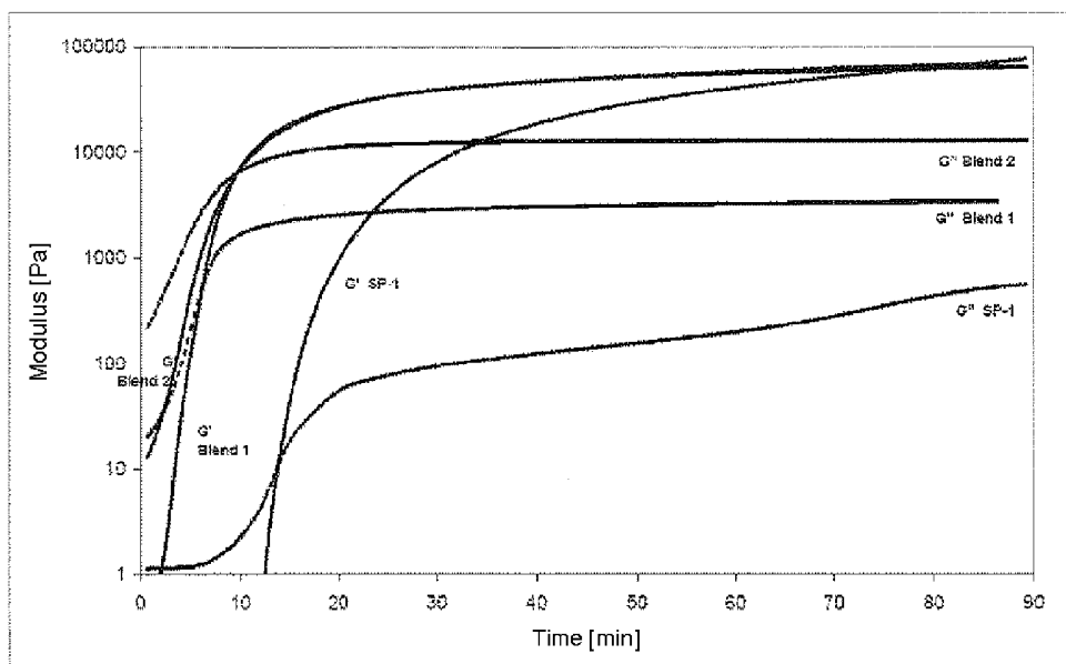
Figure 2: Oscillation rheology studies of SP-1, blend 1 and blend 2 in comparison
