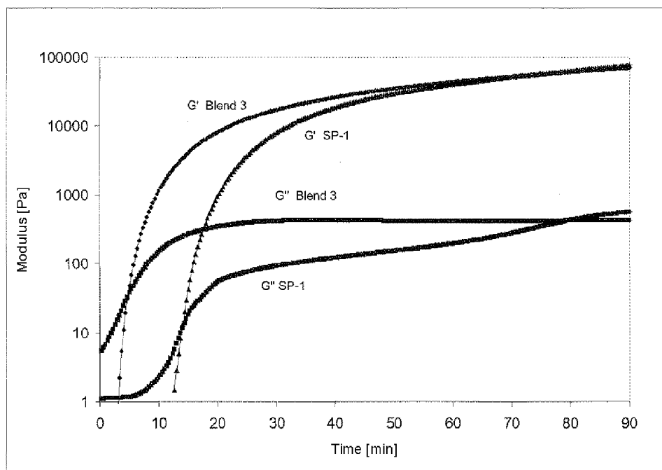
Figure 3: Oscillation rheology studies of SP-1 and blend 3 in comparison
