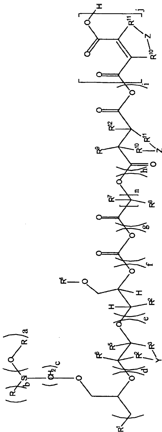
Figure 1: Structure of the formula (1)
