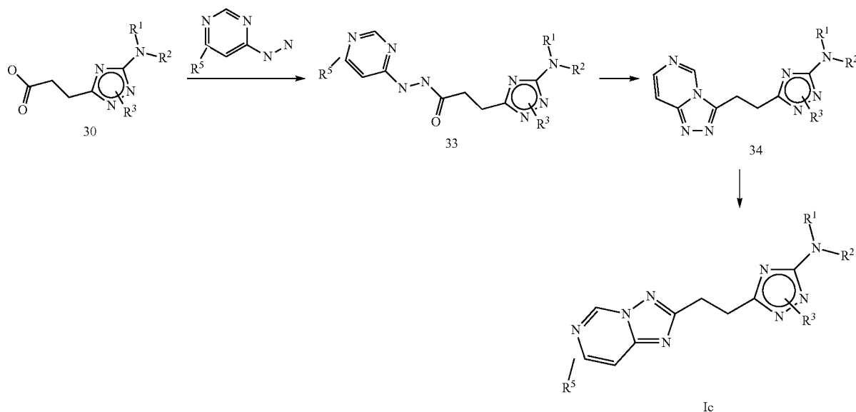
Scheme 8
