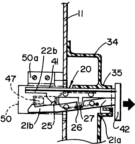
SWITCH "OFF"
