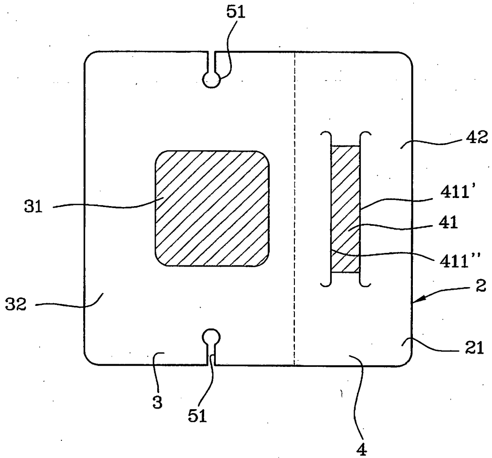
back view
