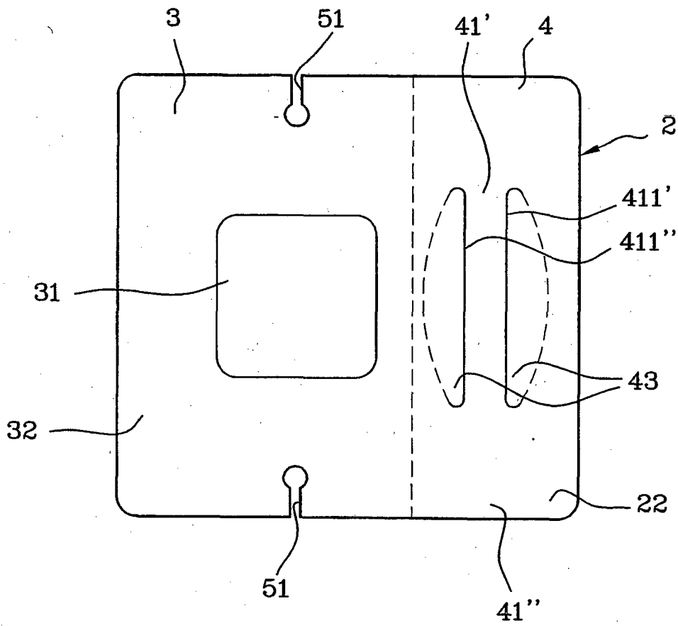
top view
