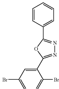
2-(2,5-Dibromo-phenyl)-5-phenyl-[1,3,4]oxadiazole,
