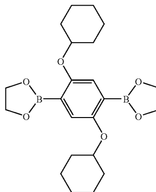
2-(4-[1,3,2]Dioxaborolan-2-yl)-2,5 dicyclohexyloxy-phenyl-[1,3,2]dioxaborolane
