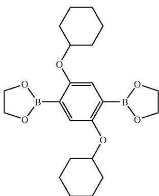
2-(4-[1,3,2]Dioxaborolan-2-yl-2,5-dicyclohexyloxy-phenyl)-[1,3,2]dioxaborolane
