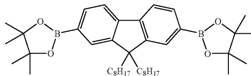
9,9-Dioctylfluorene-2,7-bis(pinacol boronate),
