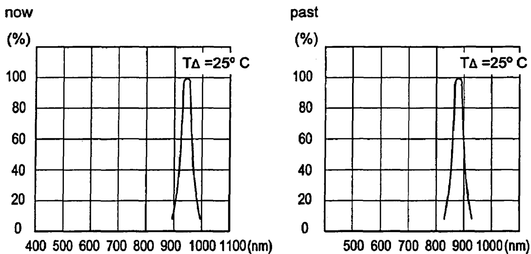
The spectral curve of the LED
