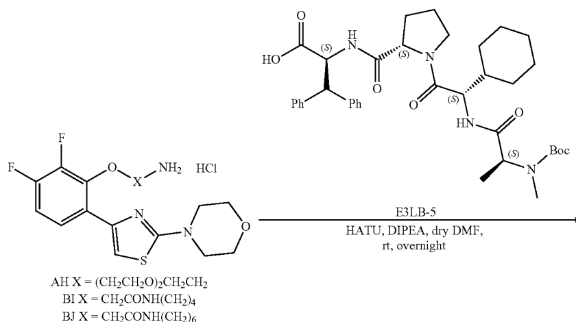
Scheme 13. Synthesis of Examples 24-26
