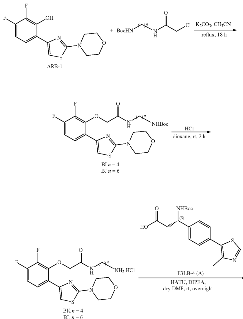
Scheme 11. Synthesis of Examples 22 and 23.
