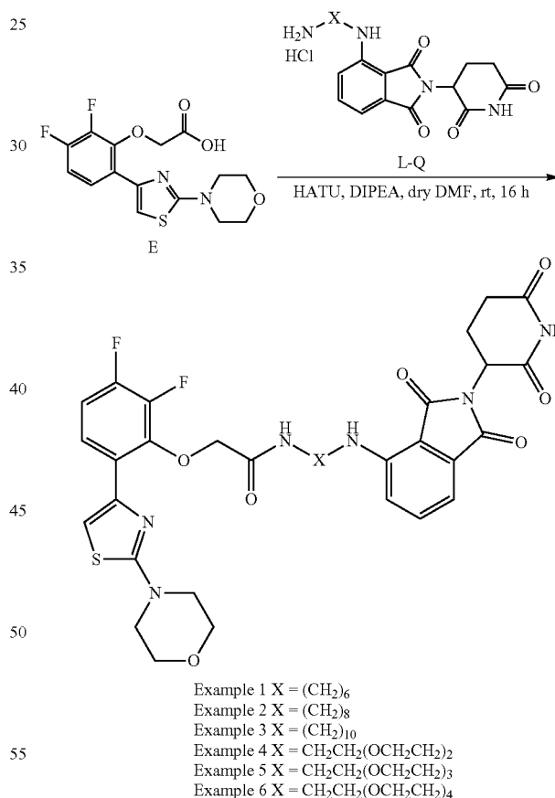
Scheme 3. Synthesis of Examples 1-6
