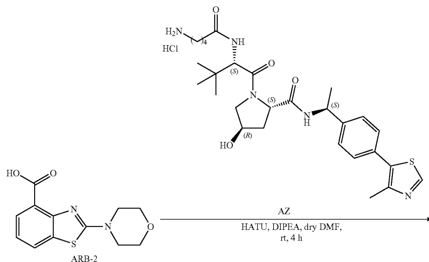
Scheme 16. Synthesis of Examples 30.
