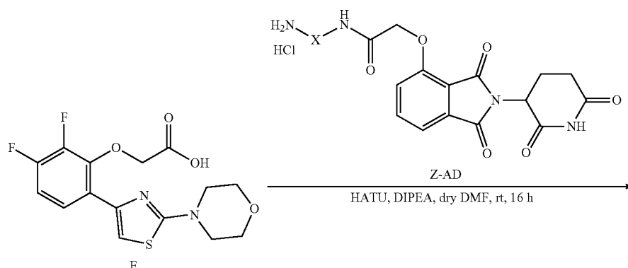
Scheme 5. Synthesis of Examples 7-11.
