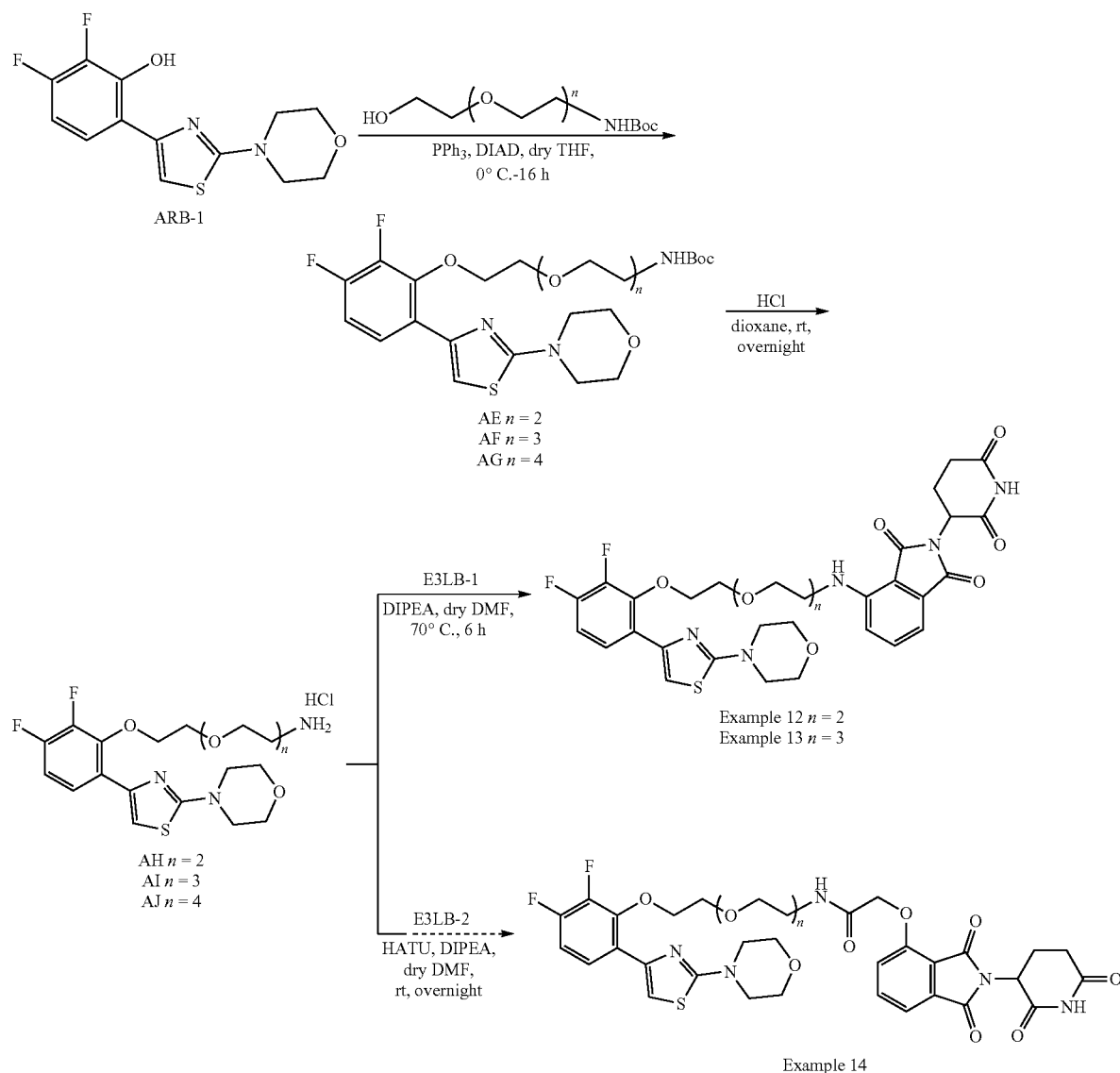
Scheme 6. Synthesis of Examples 12-14.
