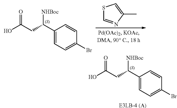
Scheme 10. Synthesis of VHL-based E3LB-4 moieties.
