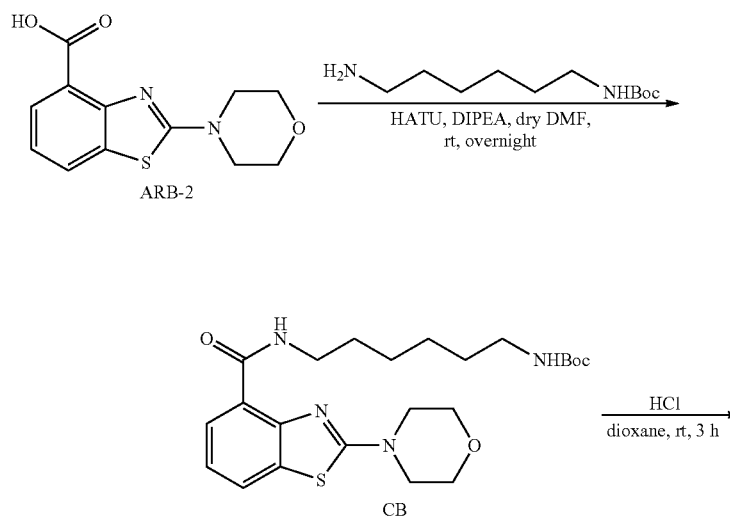
Scheme 17. Synthesis of Examples 31.
