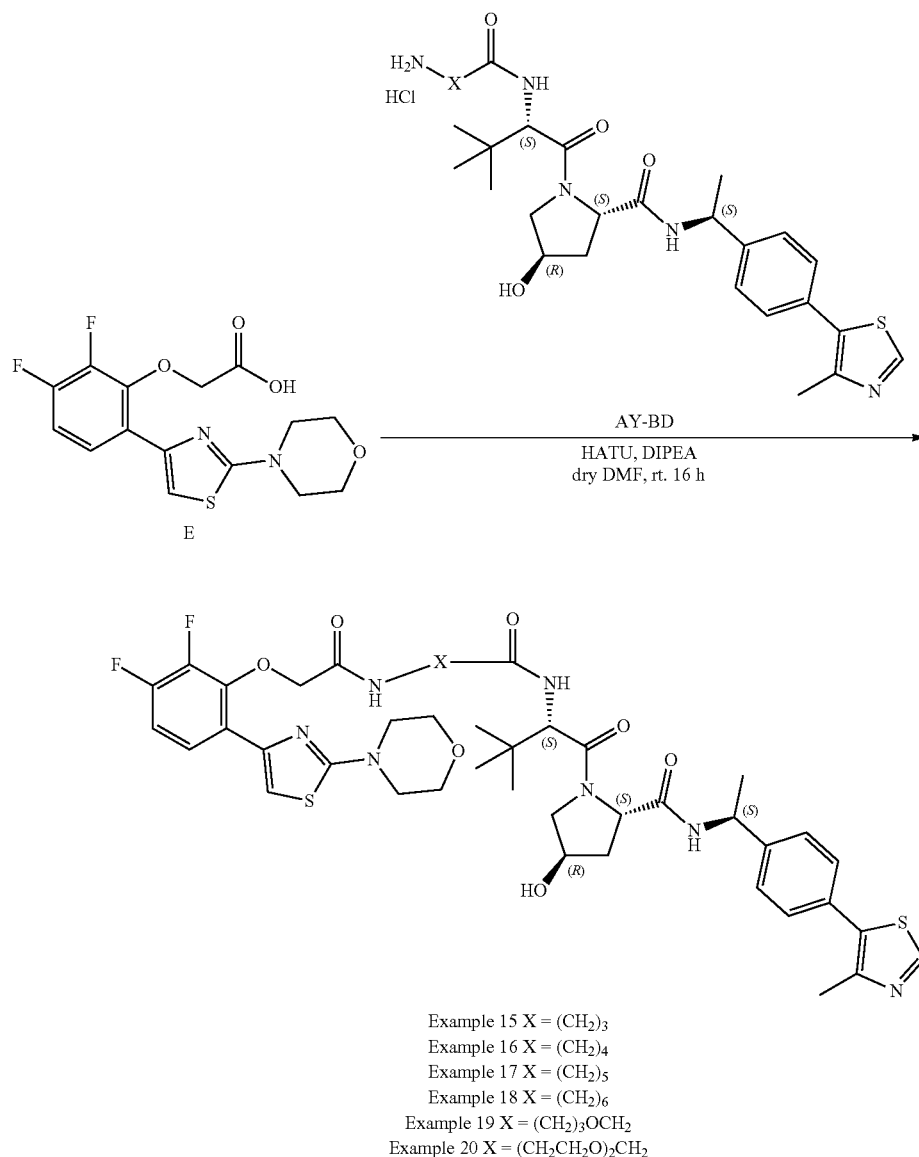
Scheme 8. Synthesis Examples 15-20.
