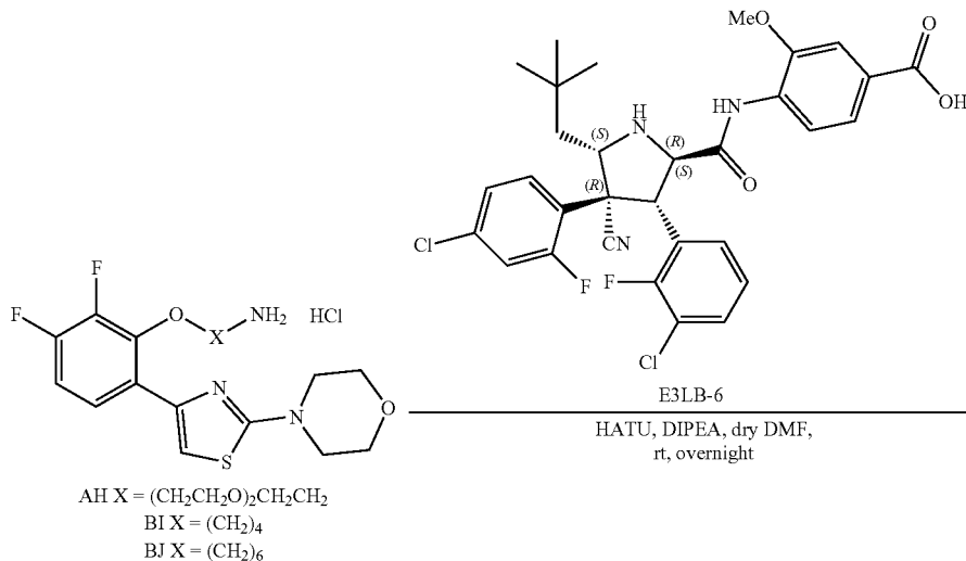
Scheme 14. Synthesis of Examples 27-29.
