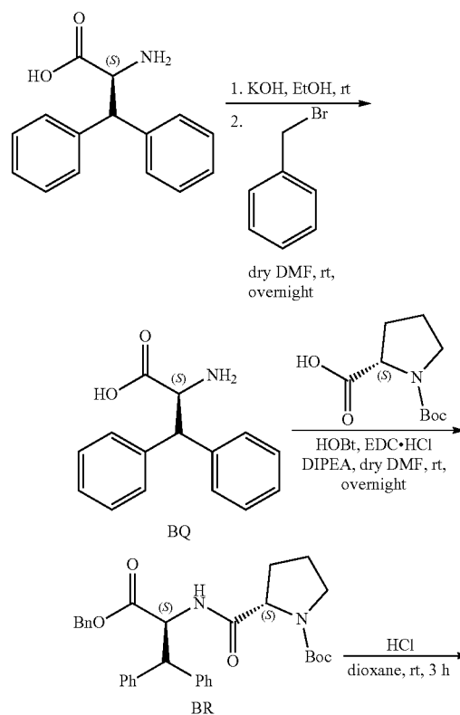
Scheme 12. Synthesis of IAP ligand-based E3LB-5 moiety.
