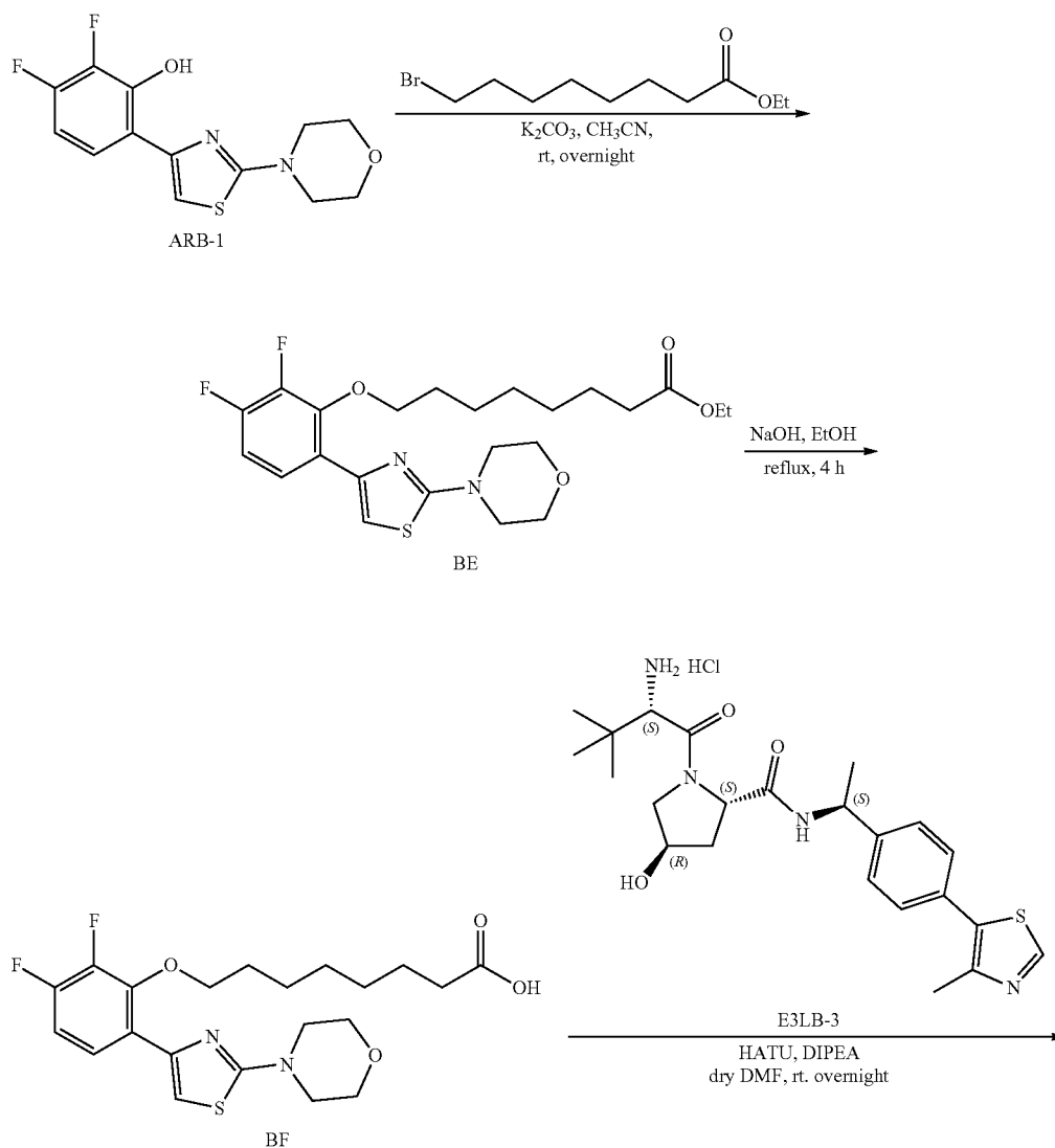
Scheme 9. Synthesis of Example 21.
