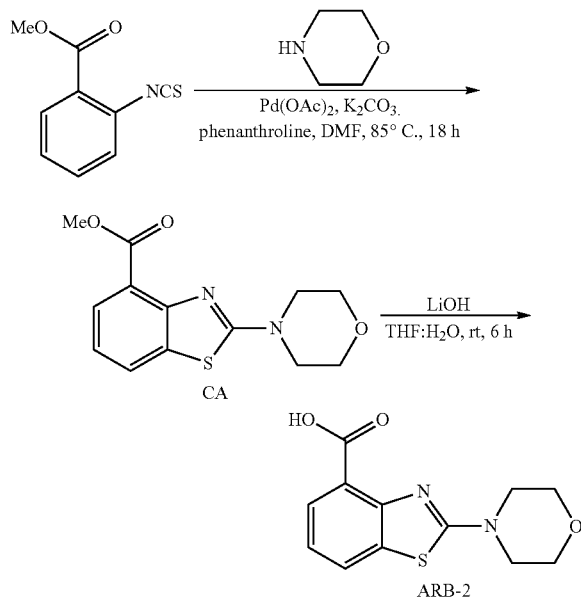
Scheme 15. Synthesis of ARB-2 moiety.
