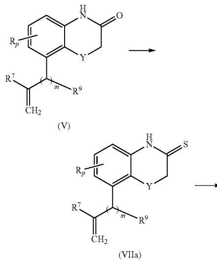
Scheme 5
