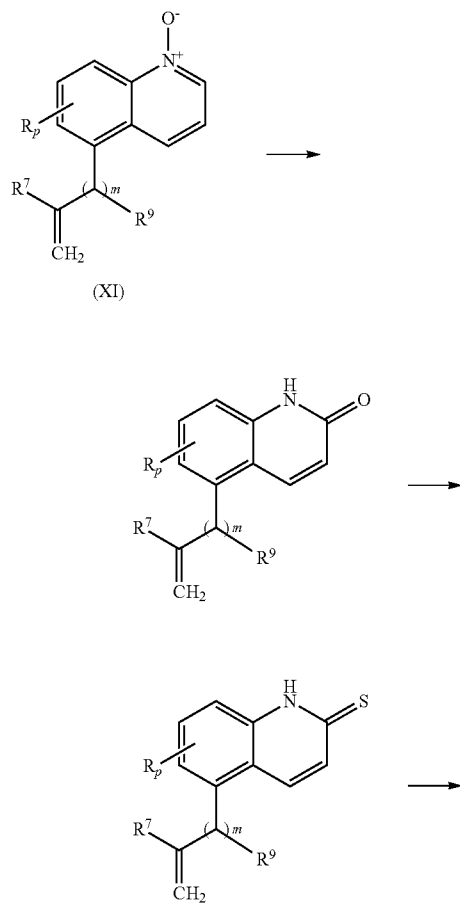
Scheme 12
