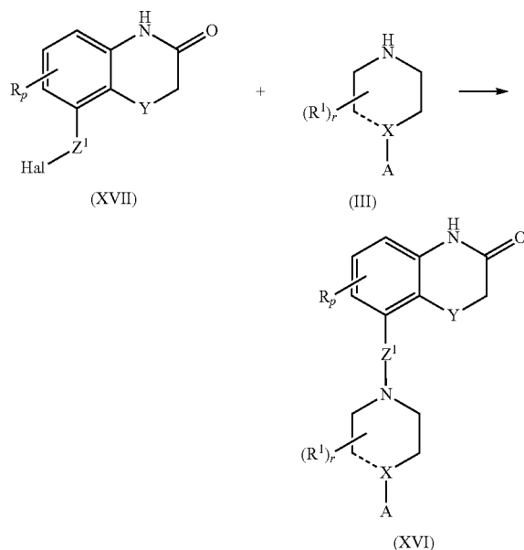
Scheme 20
