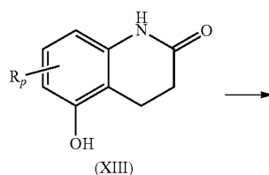
Scheme 16
