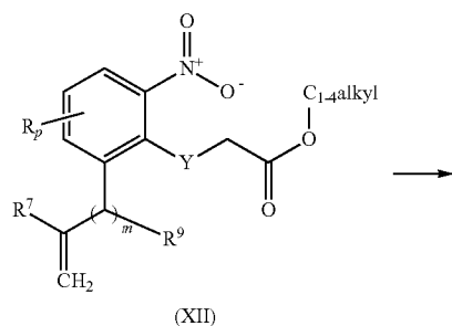
Scheme 14
