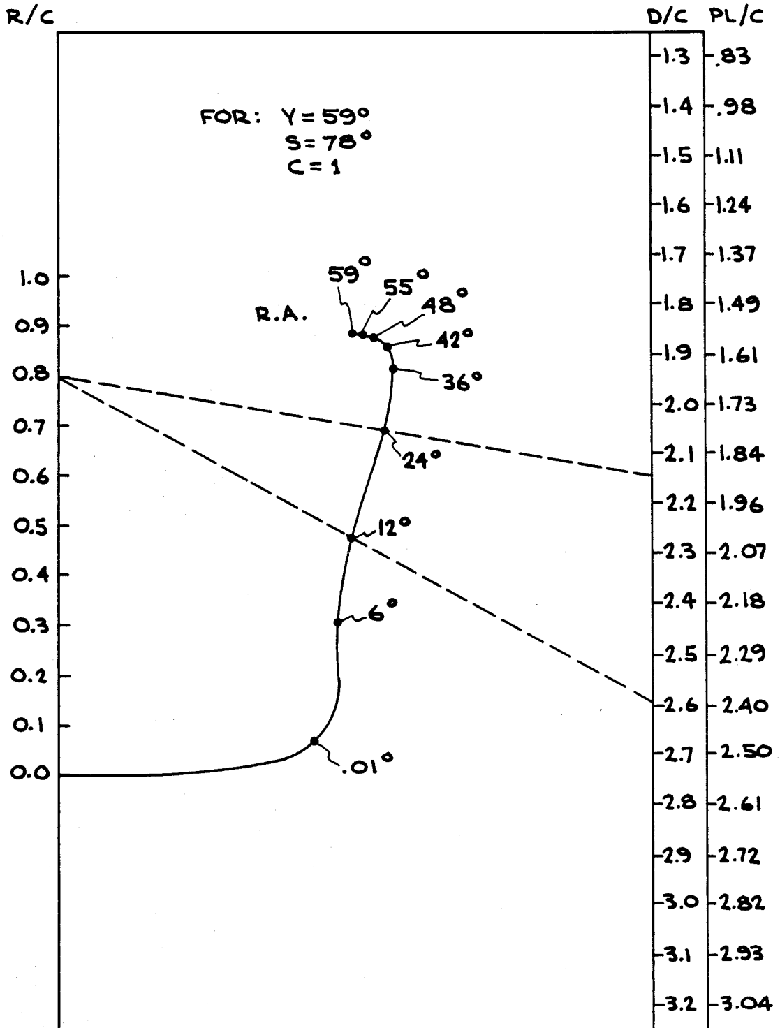
ALIGNMENT CHART FOR 3 VARIABLES (R/C, D/C OR PL/C, RA) HAVING Y, S, C AS CONSTANTS FROM FORMULA 1
