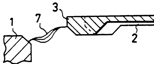
FIG. 5 (c) (Prior Art)
