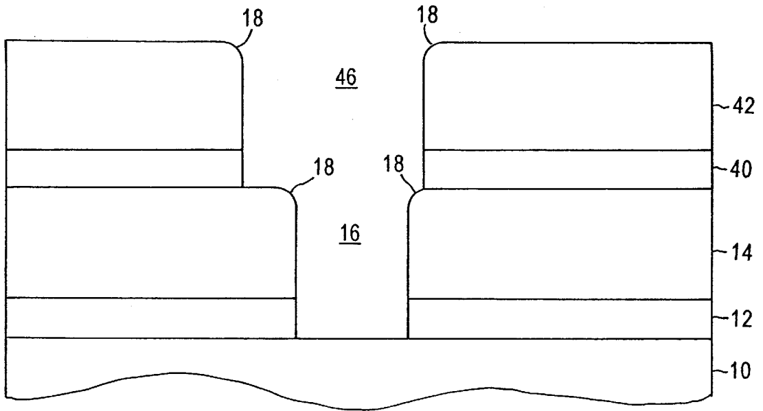
FIG. 2I (PRIOR ART)
