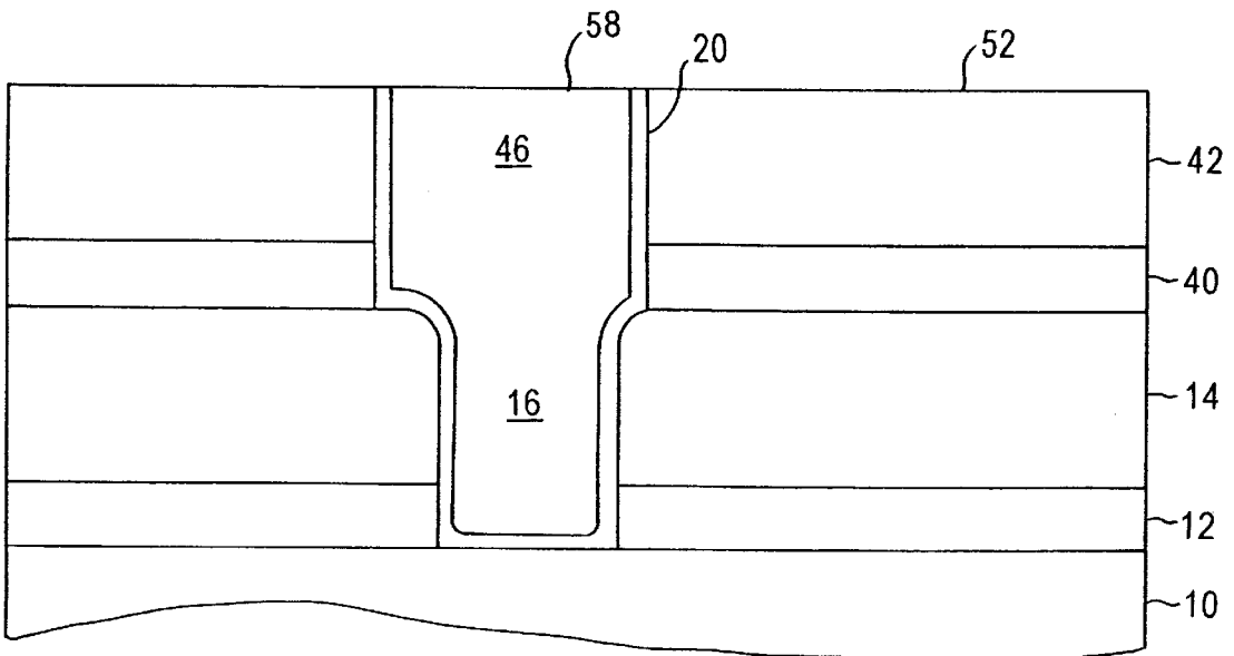
FIG. 2L (PRIOR ART)
