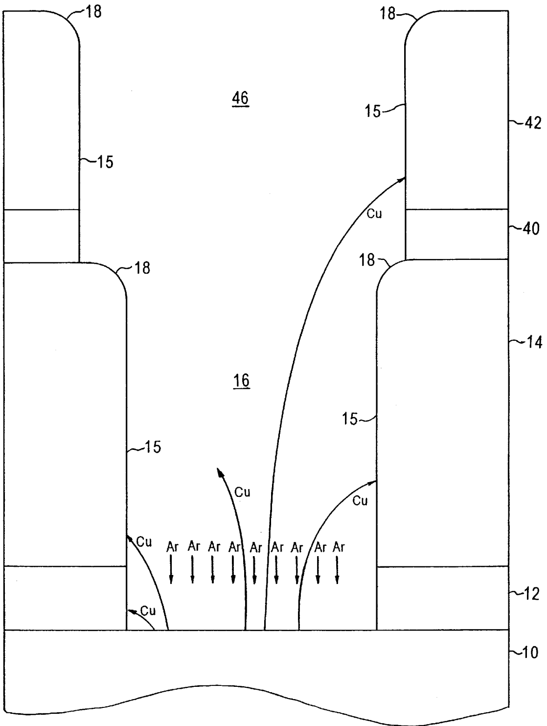
FIG. 3 (PRIOR ART)
