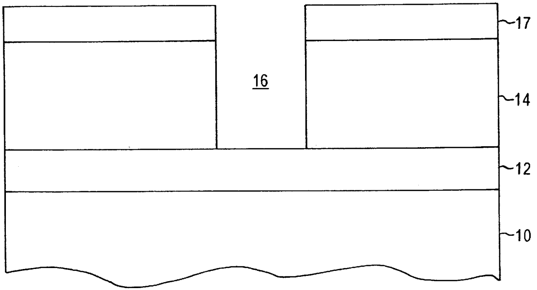
FIG. 1C (PRIOR ART)
